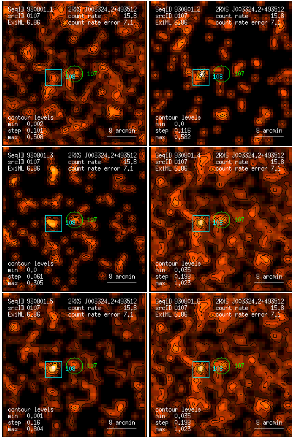
Figure 107: RASS 930801: detection 0107: band rate images, Gaussian filter: (1) PSPC channels 11 – 41, (2) 52 – 90, (3) 91 – 201, (4) 11 – 235, (5) 52 – 201, (6) 11 – 201. Broad band rates in counts/ks. Band rate contour levels in counts/ks/arcmin 2 .
