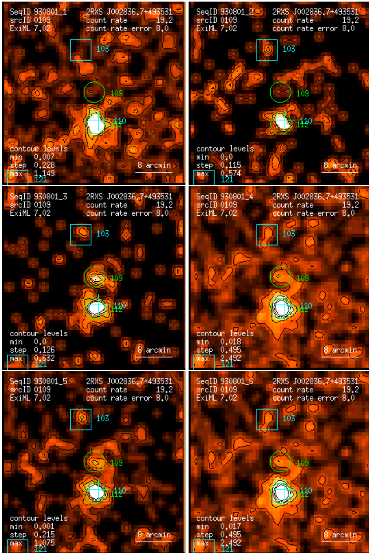
Figure 109: RASS 930801: detection 0109: band rate images, Gaussian filter: (1) PSPC channels 11 – 41, (2) 52 – 90, (3) 91 – 201, (4) 11 – 235, (5) 52 – 201, (6) 11 – 201. Broad band rates in counts/ks. Band rate contour levels in counts/ks/arcmin 2 .
