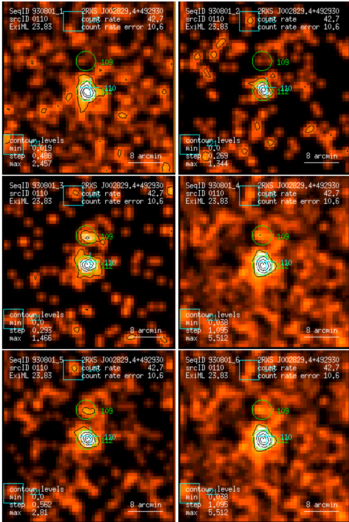
Figure 110: RASS 930801: detection 0110: band rate images, Gaussian filter: (1) PSPC channels 11 – 41, (2) 52 – 90, (3) 91 – 201, (4) 11 – 235, (5) 52 – 201, (6) 11 – 201. Broad band rates in counts/ks. Band rate contour levels in counts/ks/arcmin 2 .
