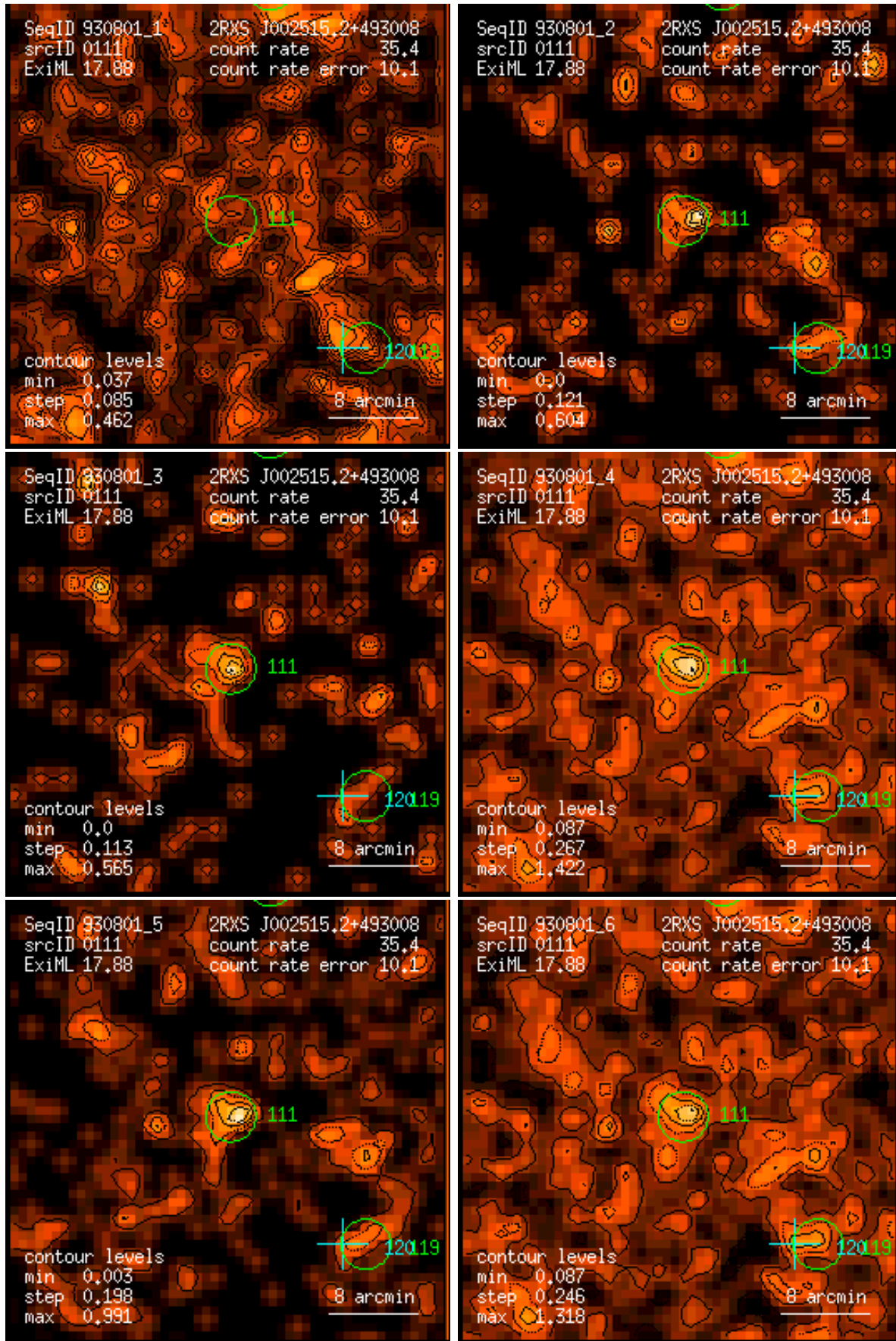
Figure 111: RASS 930801: detection 0111: band rate images, Gaussian filter: (1) PSPC channels 11 – 41, (2) 52 – 90, (3) 91 – 201, (4) 11 – 235, (5) 52 – 201, (6) 11 – 201. Broad band rates in counts/ks. Band rate contour levels in counts/ks/arcmin 2 .
