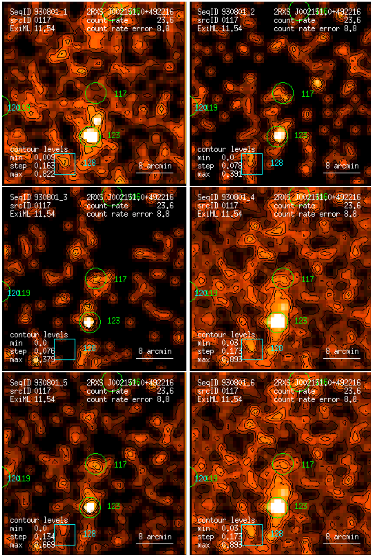
Figure 117: RASS 930801: detection 0117: band rate images, Gaussian filter: (1) PSPC channels 11 – 41, (2) 52 – 90, (3) 91 – 201, (4) 11 – 235, (5) 52 – 201, (6) 11 – 201. Broad band rates in counts/ks. Band rate contour levels in counts/ks/arcmin 2 .
