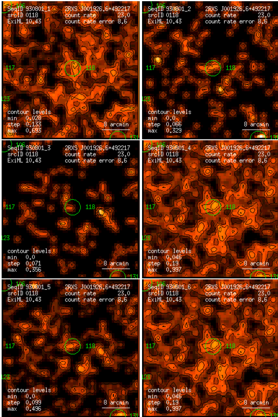
Figure 118: RASS 930801: detection 0118: band rate images, Gaussian filter: (1) PSPC channels 11 – 41, (2) 52 – 90, (3) 91 – 201, (4) 11 – 235, (5) 52 – 201, (6) 11 – 201. Broad band rates in counts/ks. Band rate contour levels in counts/ks/arcmin 2 .
