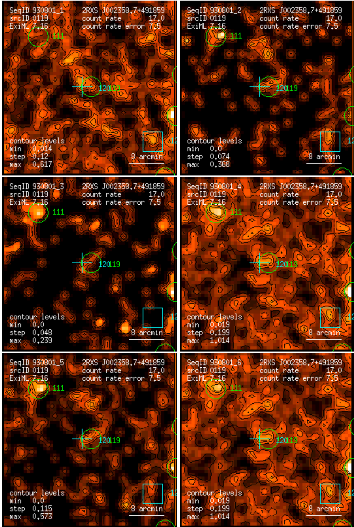
Figure 119: RASS 930801: detection 0119: band rate images, Gaussian filter: (1) PSPC channels 11 – 41, (2) 52 – 90, (3) 91 – 201, (4) 11 – 235, (5) 52 – 201, (6) 11 – 201. Broad band rates in counts/ks. Band rate contour levels in counts/ks/arcmin 2 .
