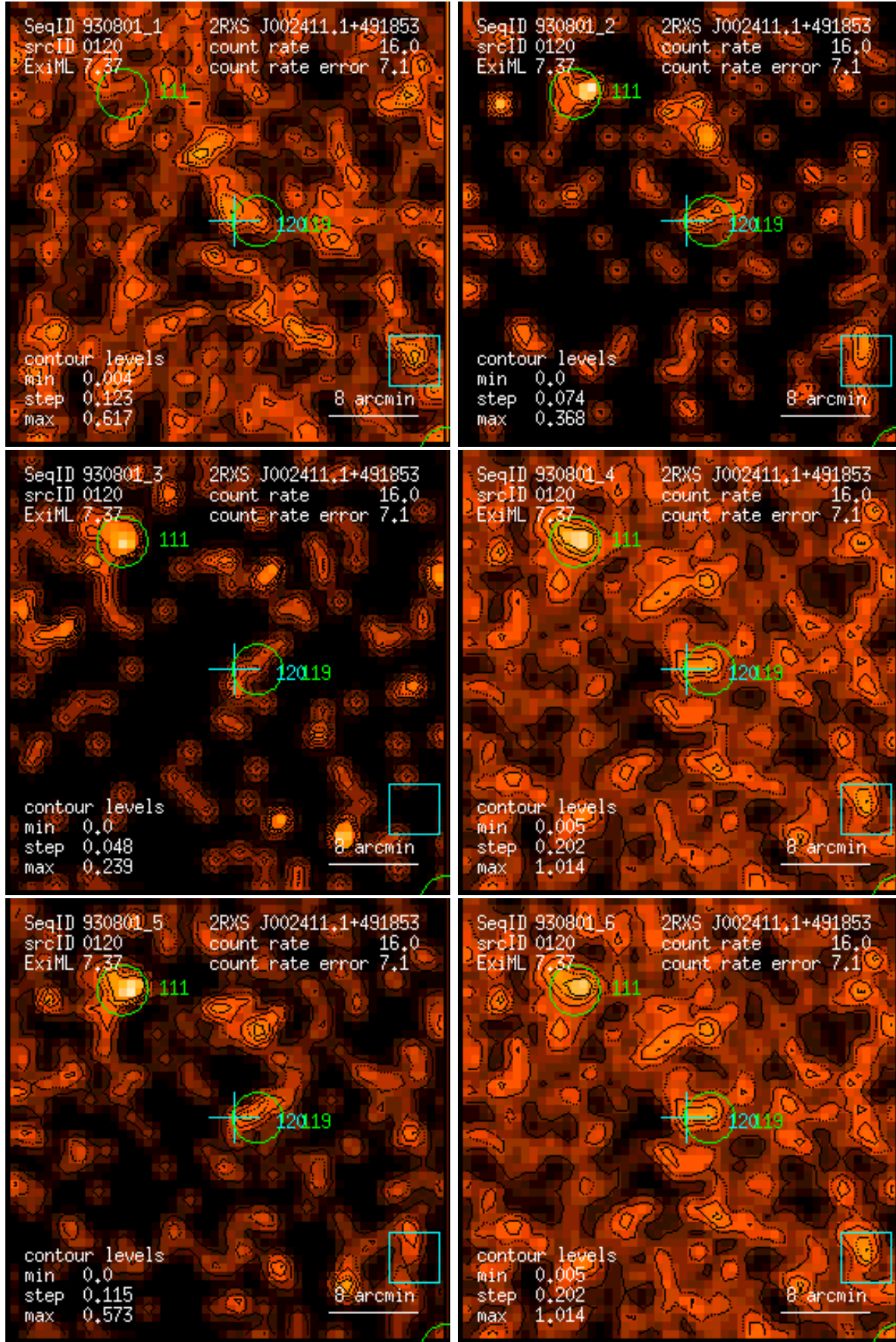
Figure 120: RASS 930801: detection 0120: band rate images, Gaussian filter: (1) PSPC channels 11 – 41, (2) 52 – 90, (3) 91 – 201, (4) 11 – 235, (5) 52 – 201, (6) 11 – 201. Broad band rates in counts/ks. Band rate contour levels in counts/ks/arcmin 2 .
