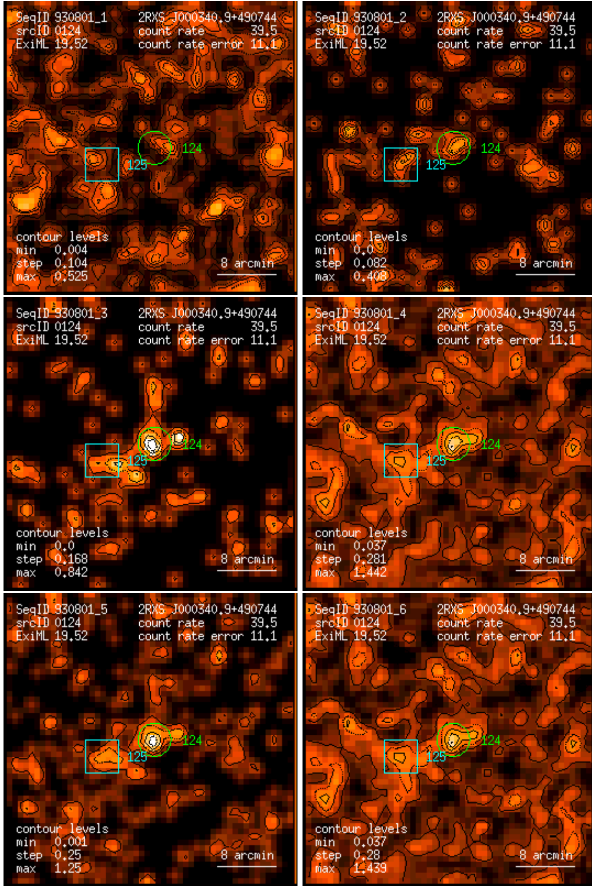
Figure 124: RASS 930801: detection 0124: band rate images, Gaussian filter: (1) PSPC channels 11 – 41, (2) 52 – 90, (3) 91 – 201, (4) 11 – 235, (5) 52 – 201, (6) 11 – 201. Broad band rates in counts/ks. Band rate contour levels in counts/ks/arcmin 2 .
