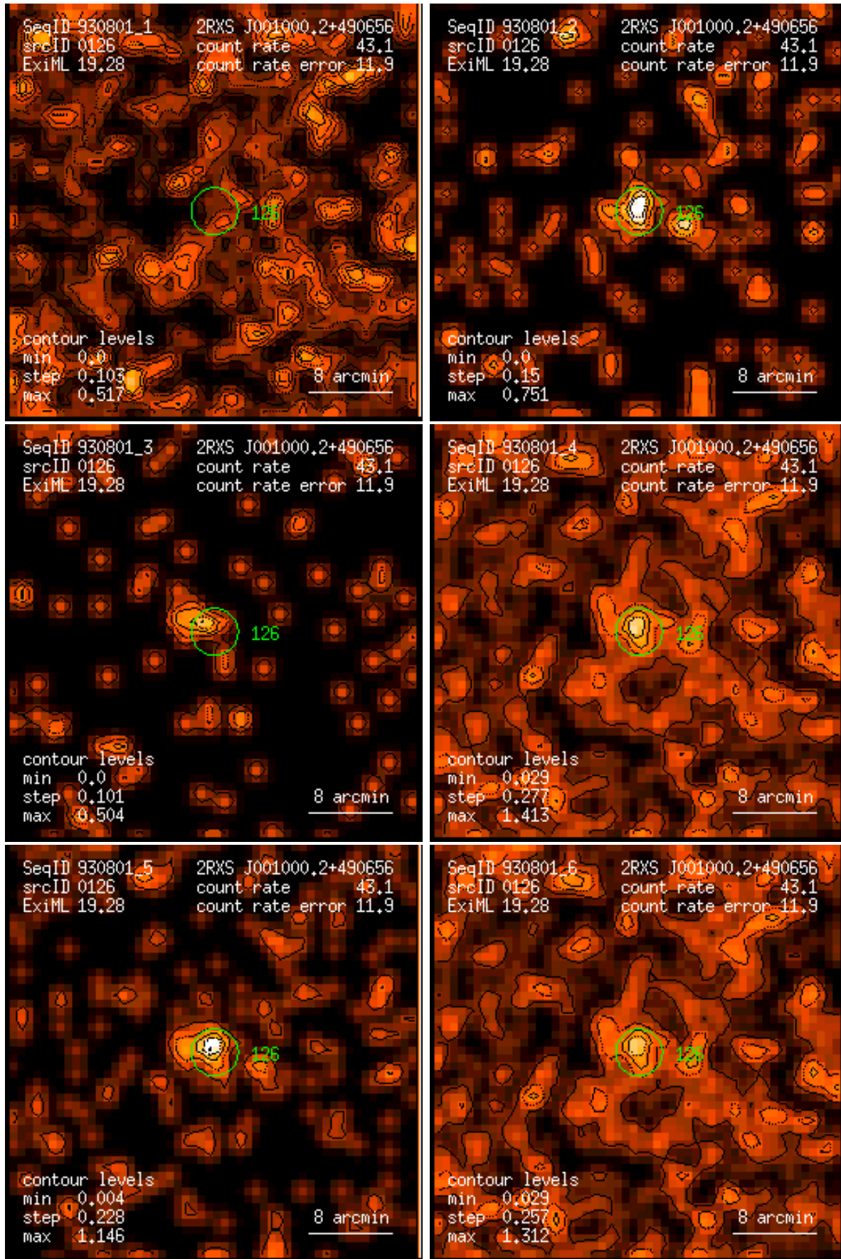
Figure 126: RASS 930801: detection 0126: band rate images, Gaussian filter: (1) PSPC channels 11 – 41, (2) 52 – 90, (3) 91 – 201, (4) 11 – 235, (5) 52 – 201, (6) 11 – 201. Broad band rates in counts/ks. Band rate contour levels in counts/ks/arcmin 2 .
