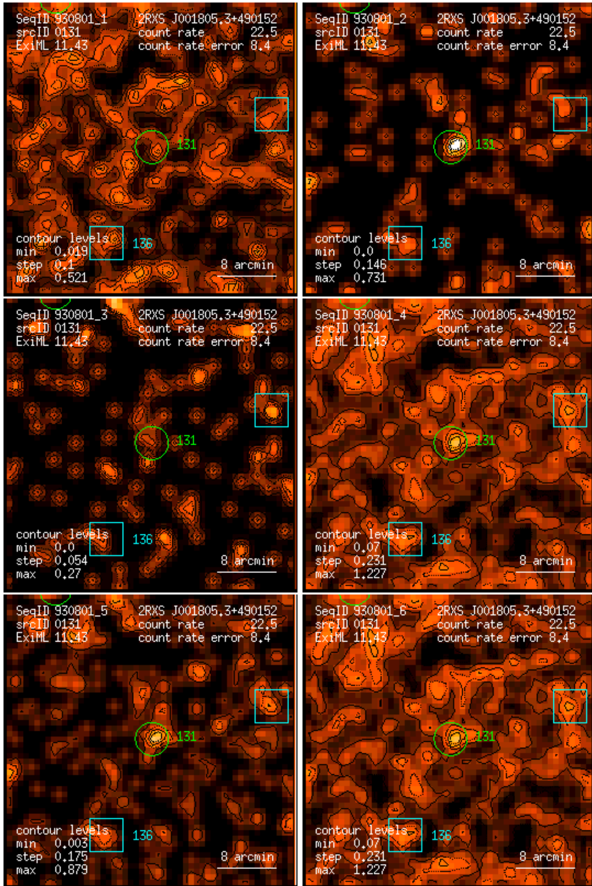
Figure 131: RASS 930801: detection 0131: band rate images, Gaussian filter: (1) PSPC channels 11 – 41, (2) 52 – 90, (3) 91 – 201, (4) 11 – 235, (5) 52 – 201, (6) 11 – 201. Broad band rates in counts/ks. Band rate contour levels in counts/ks/arcmin 2 .
