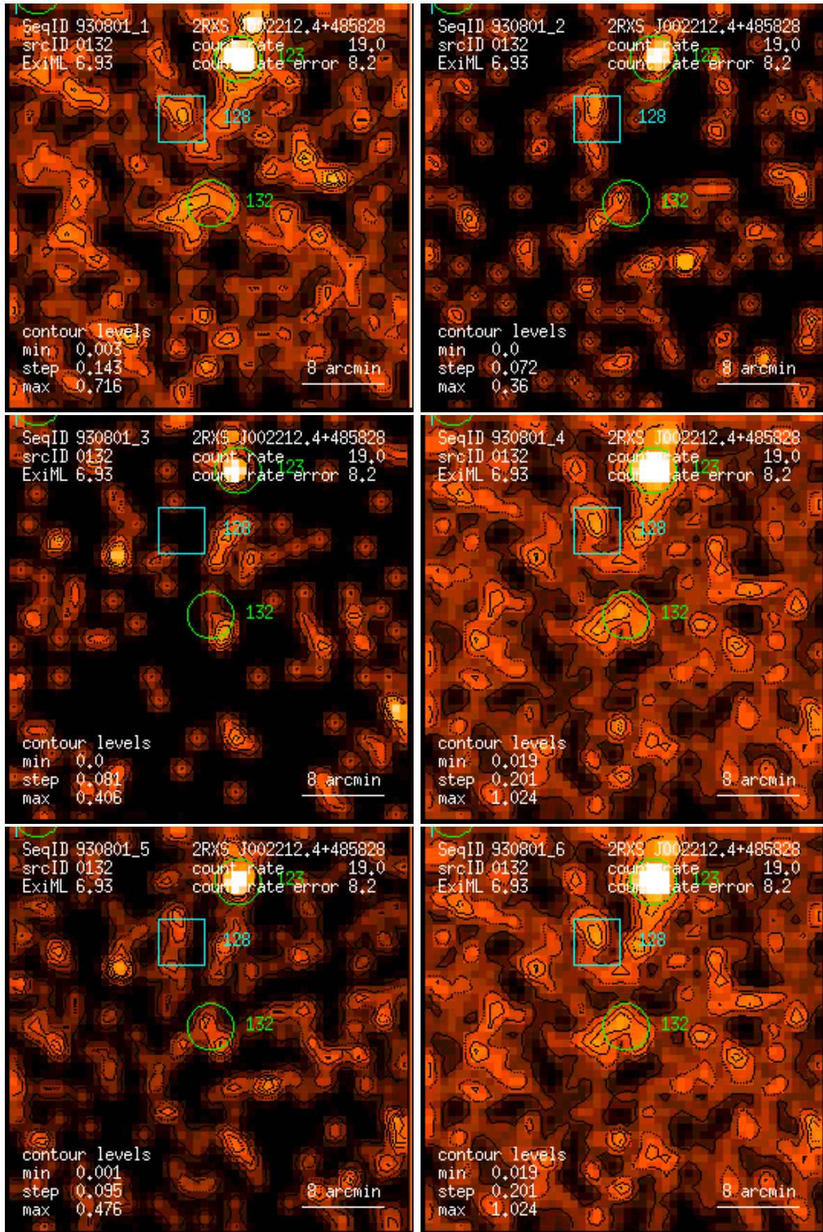
Figure 132: RASS 930801: detection 0132: band rate images, Gaussian filter: (1) PSPC channels 11 – 41, (2) 52 – 90, (3) 91 – 201, (4) 11 – 235, (5) 52 – 201, (6) 11 – 201. Broad band rates in counts/ks. Band rate contour levels in counts/ks/arcmin 2 .
