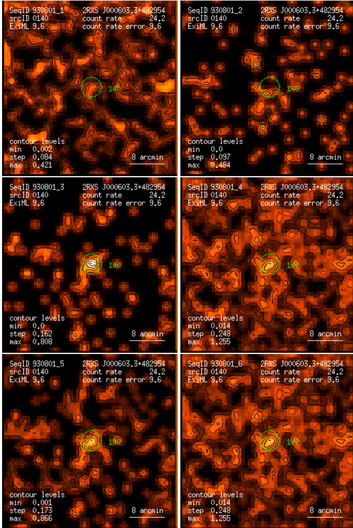
Figure 140: RASS 930801: detection 0140: band rate images, Gaussian filter: (1) PSPC channels 11 – 41, (2) 52 – 90, (3) 91 – 201, (4) 11 – 235, (5) 52 – 201, (6) 11 – 201. Broad band rates in counts/ks. Band rate contour levels in counts/ks/arcmin 2 .
