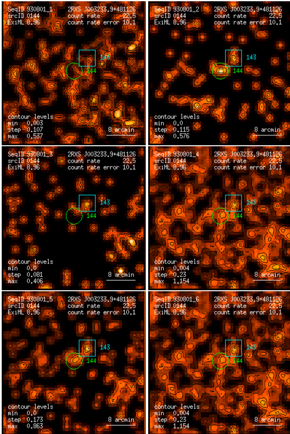
Figure 144: RASS 930801: detection 0144: band rate images, Gaussian filter: (1) PSPC channels 11 – 41, (2) 52 – 90, (3) 91 – 201, (4) 11 – 235, (5) 52 – 201, (6) 11 – 201. Broad band rates in counts/ks. Band rate contour levels in counts/ks/arcmin 2 .
