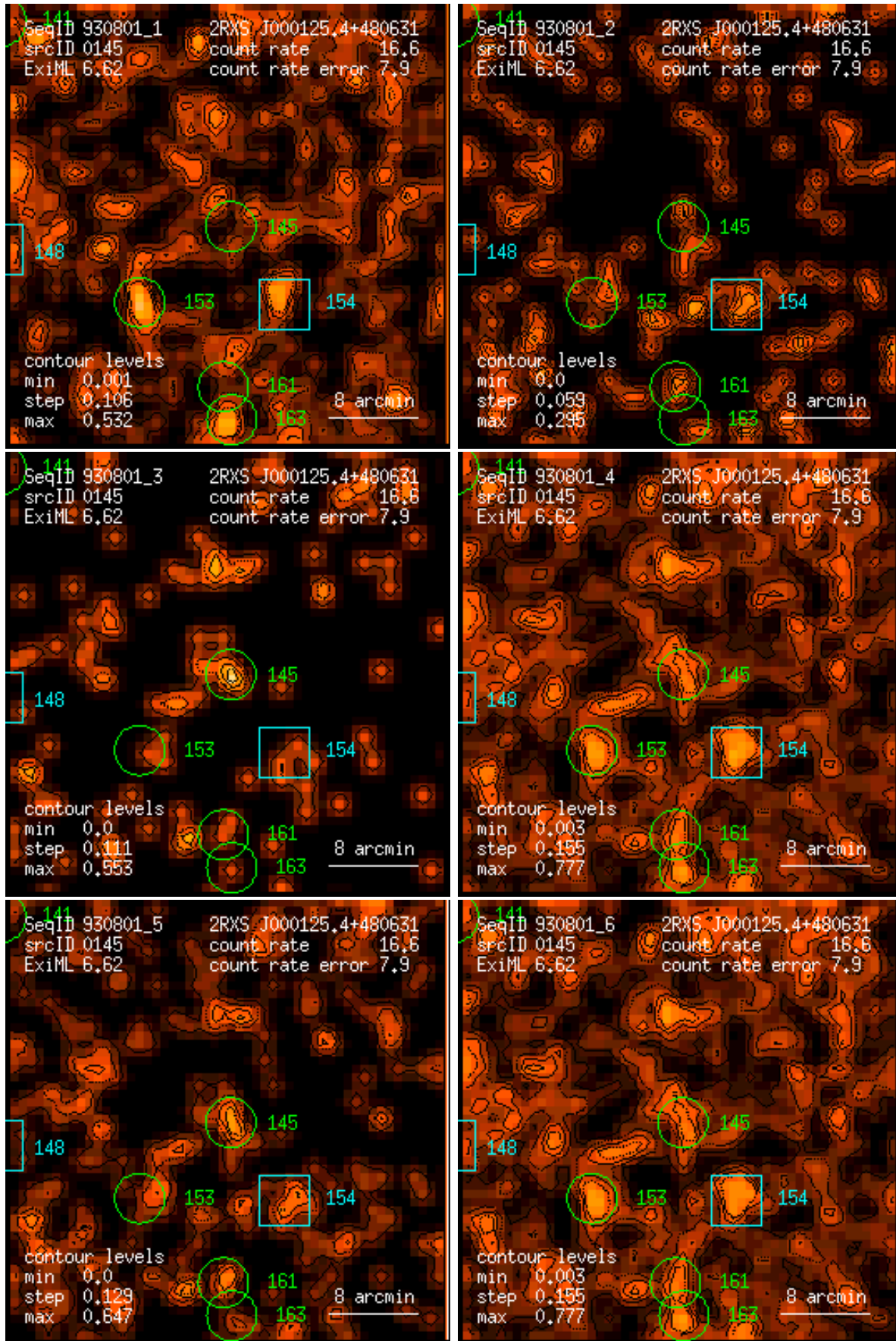
Figure 145: RASS 930801: detection 0145: band rate images, Gaussian filter: (1) PSPC channels 11 – 41, (2) 52 – 90, (3) 91 – 201, (4) 11 – 235, (5) 52 – 201, (6) 11 – 201. Broad band rates in counts/ks. Band rate contour levels in counts/ks/arcmin 2 .
