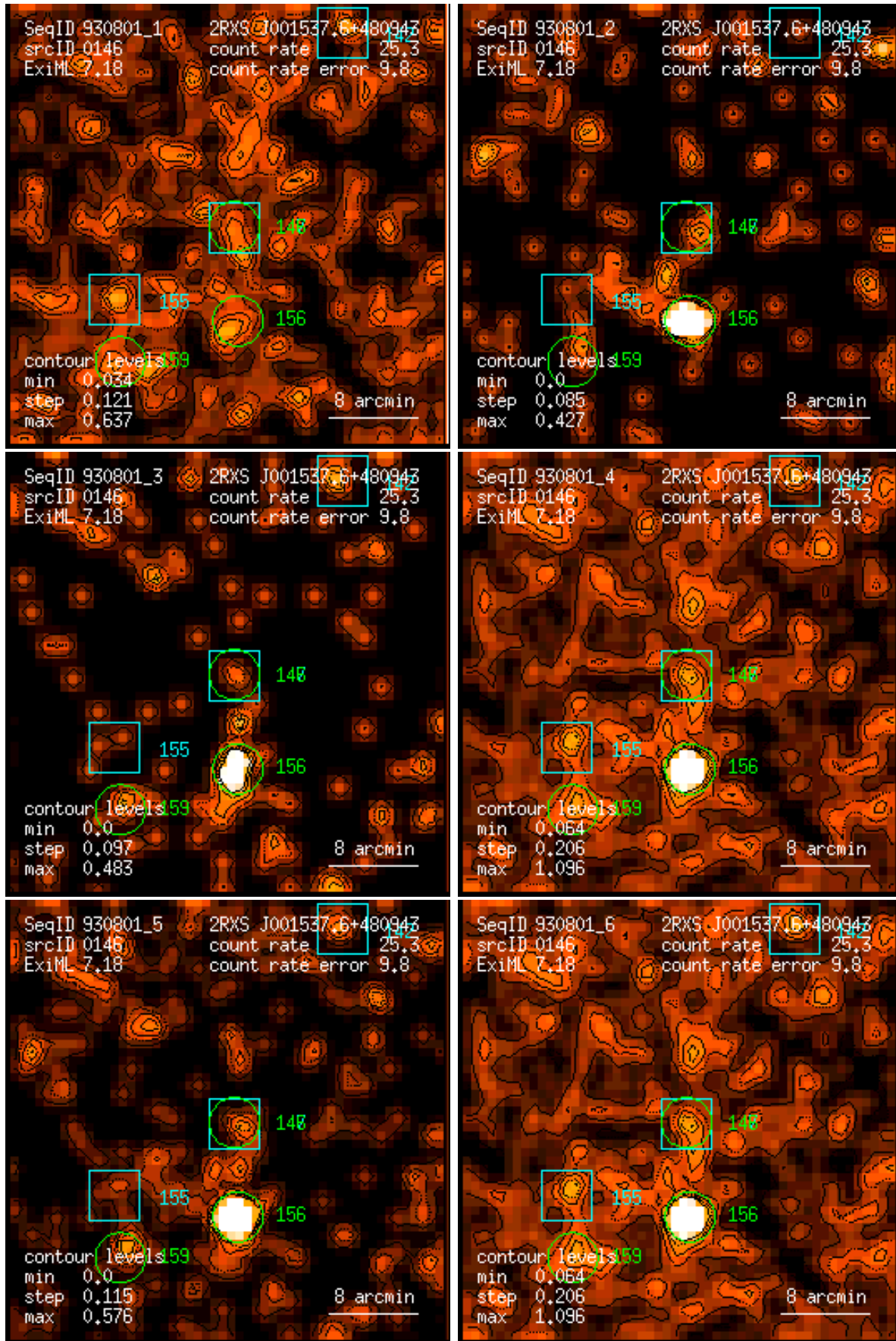
Figure 146: RASS 930801: detection 0146: band rate images, Gaussian filter: (1) PSPC channels 11 – 41, (2) 52 – 90, (3) 91 – 201, (4) 11 – 235, (5) 52 – 201, (6) 11 – 201. Broad band rates in counts/ks. Band rate contour levels in counts/ks/arcmin 2 .
