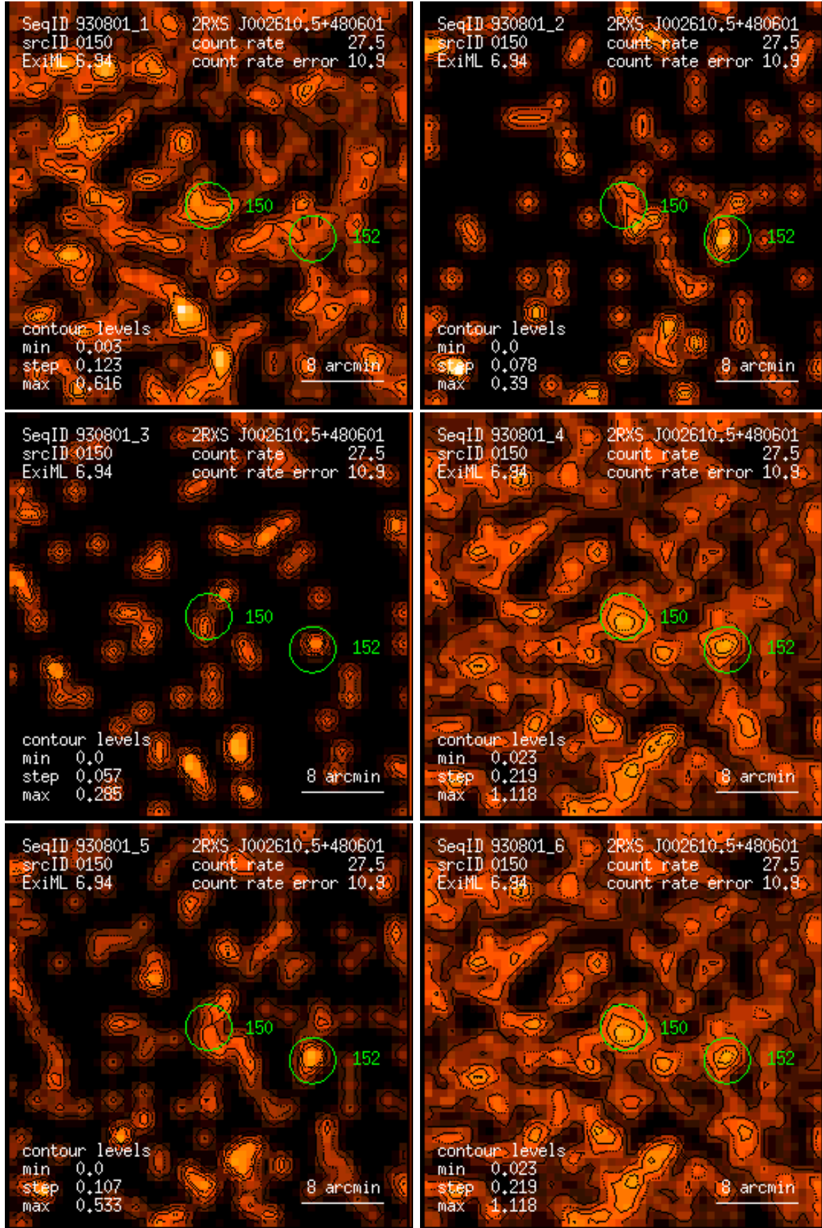
Figure 150: RASS 930801: detection 0150: band rate images, Gaussian filter: (1) PSPC channels 11 – 41, (2) 52 – 90, (3) 91 – 201, (4) 11 – 235, (5) 52 – 201, (6) 11 – 201. Broad band rates in counts/ks. Band rate contour levels in counts/ks/arcmin 2 .
