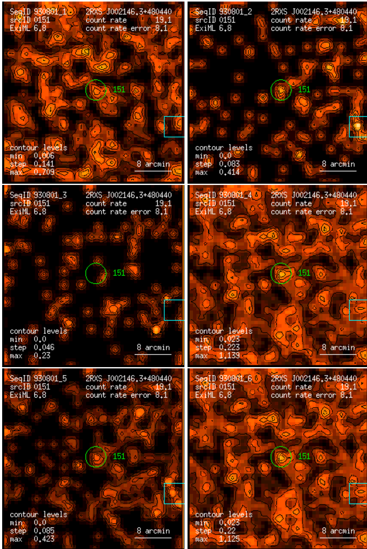
Figure 151: RASS 930801: detection 0151: band rate images, Gaussian filter: (1) PSPC channels 11 – 41, (2) 52 – 90, (3) 91 – 201, (4) 11 – 235, (5) 52 – 201, (6) 11 – 201. Broad band rates in counts/ks. Band rate contour levels in counts/ks/arcmin 2 .
