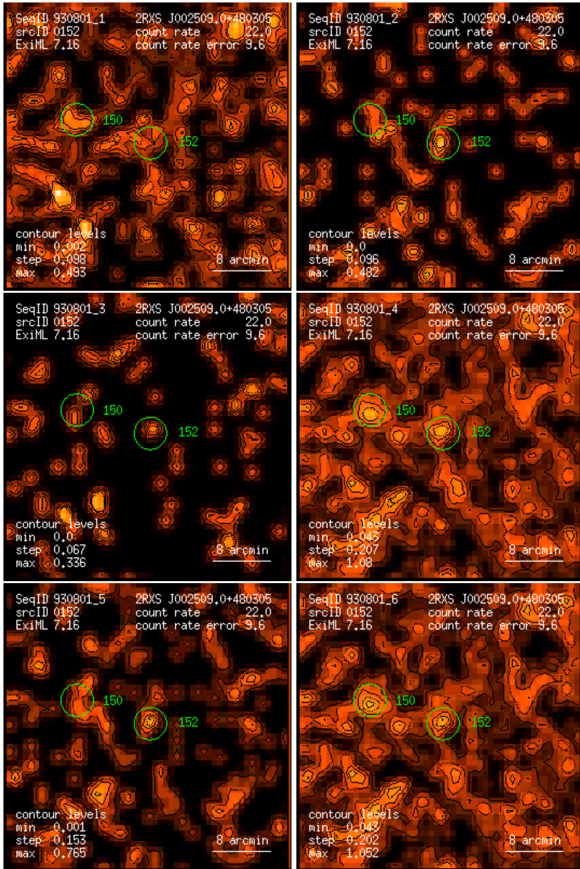
Figure 152: RASS 930801: detection 0152: band rate images, Gaussian filter: (1) PSPC channels 11 – 41, (2) 52 – 90, (3) 91 – 201, (4) 11 – 235, (5) 52 – 201, (6) 11 – 201. Broad band rates in counts/ks. Band rate contour levels in counts/ks/arcmin 2 .
