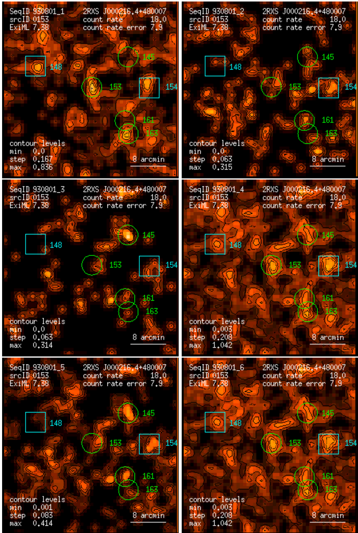
Figure 153: RASS 930801: detection 0153: band rate images, Gaussian filter: (1) PSPC channels 11 – 41, (2) 52 – 90, (3) 91 – 201, (4) 11 – 235, (5) 52 – 201, (6) 11 – 201. Broad band rates in counts/ks. Band rate contour levels in counts/ks/arcmin 2 .
