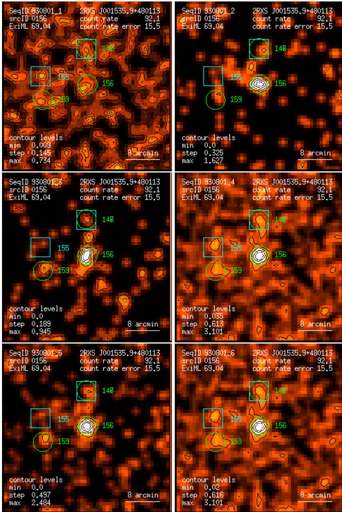
Figure 156: RASS 930801: detection 0156: band rate images, Gaussian filter: (1) PSPC channels 11 – 41, (2) 52 – 90, (3) 91 – 201, (4) 11 – 235, (5) 52 – 201, (6) 11 – 201. Broad band rates in counts/ks. Band rate contour levels in counts/ks/arcmin 2 .
