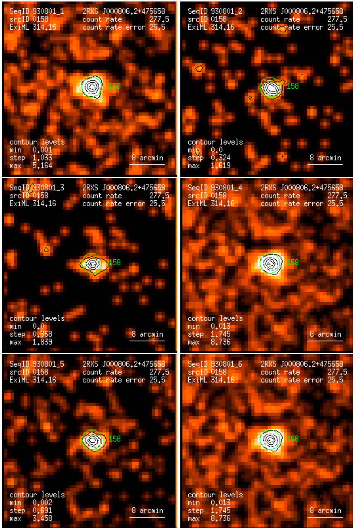
Figure 158: RASS 930801: detection 0158: band rate images, Gaussian filter: (1) PSPC channels 11 – 41, (2) 52 – 90, (3) 91 – 201, (4) 11 – 235, (5) 52 – 201, (6) 11 – 201. Broad band rates in counts/ks. Band rate contour levels in counts/ks/arcmin 2 .
