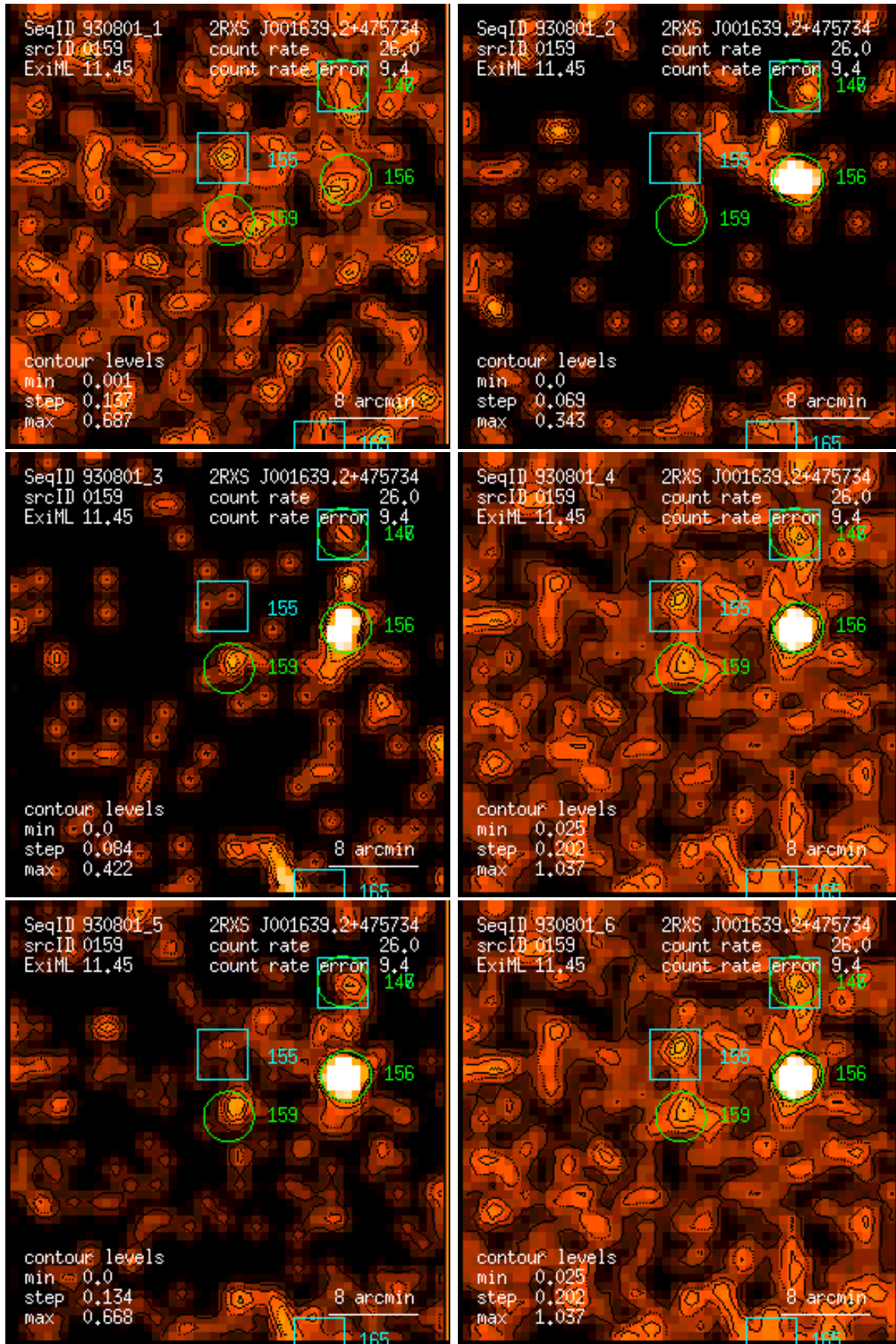
Figure 159: RASS 930801: detection 0159: band rate images, Gaussian filter: (1) PSPC channels 11 – 41, (2) 52 – 90, (3) 91 – 201, (4) 11 – 235, (5) 52 – 201, (6) 11 – 201. Broad band rates in counts/ks. Band rate contour levels in counts/ks/arcmin 2 .
