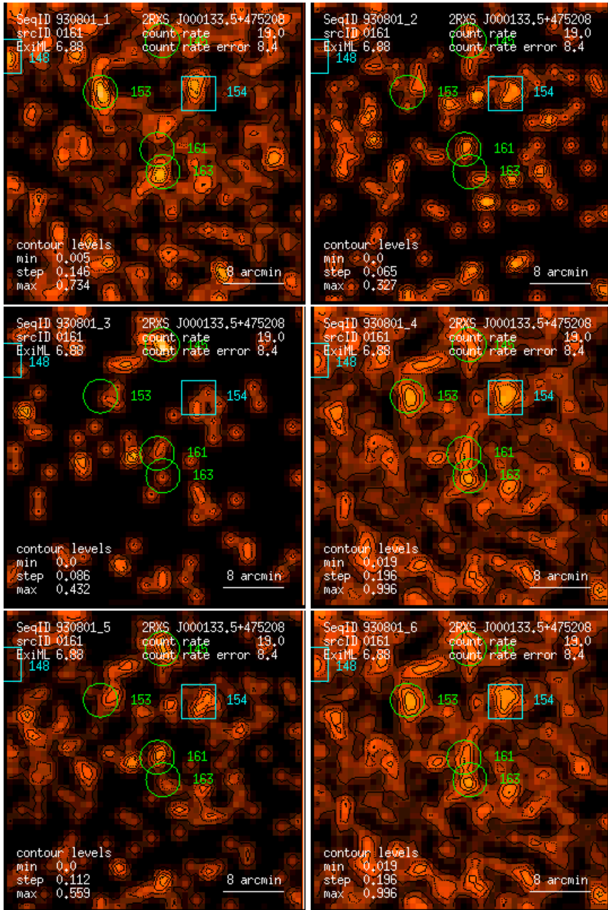
Figure 161: RASS 930801: detection 0161: band rate images, Gaussian filter: (1) PSPC channels 11 – 41, (2) 52 – 90, (3) 91 – 201, (4) 11 – 235, (5) 52 – 201, (6) 11 – 201. Broad band rates in counts/ks. Band rate contour levels in counts/ks/arcmin 2 .
