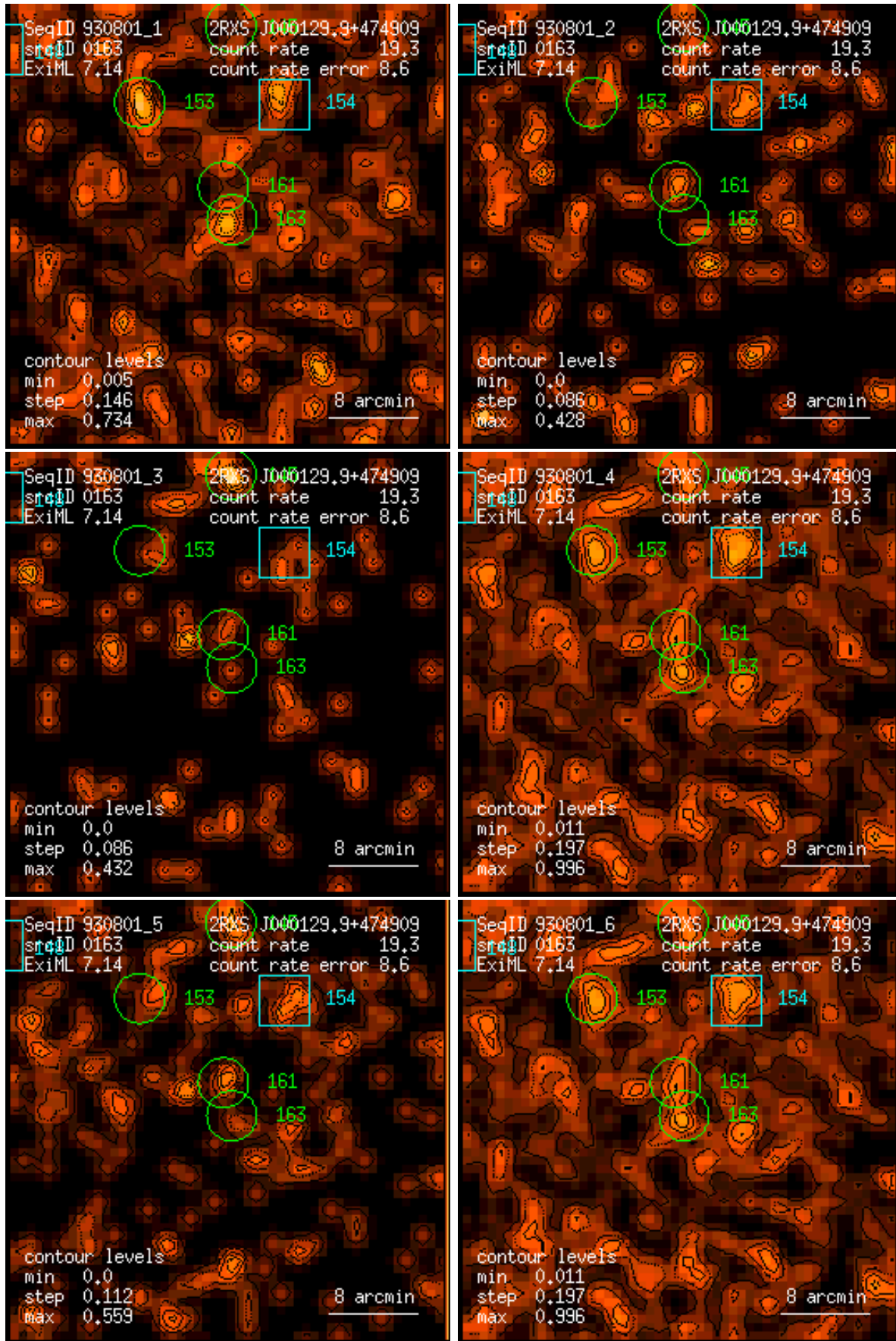
Figure 163: RASS 930801: detection 0163: band rate images, Gaussian filter: (1) PSPC channels 11 – 41, (2) 52 – 90, (3) 91 – 201, (4) 11 – 235, (5) 52 – 201, (6) 11 – 201. Broad band rates in counts/ks. Band rate contour levels in counts/ks/arcmin 2 .
