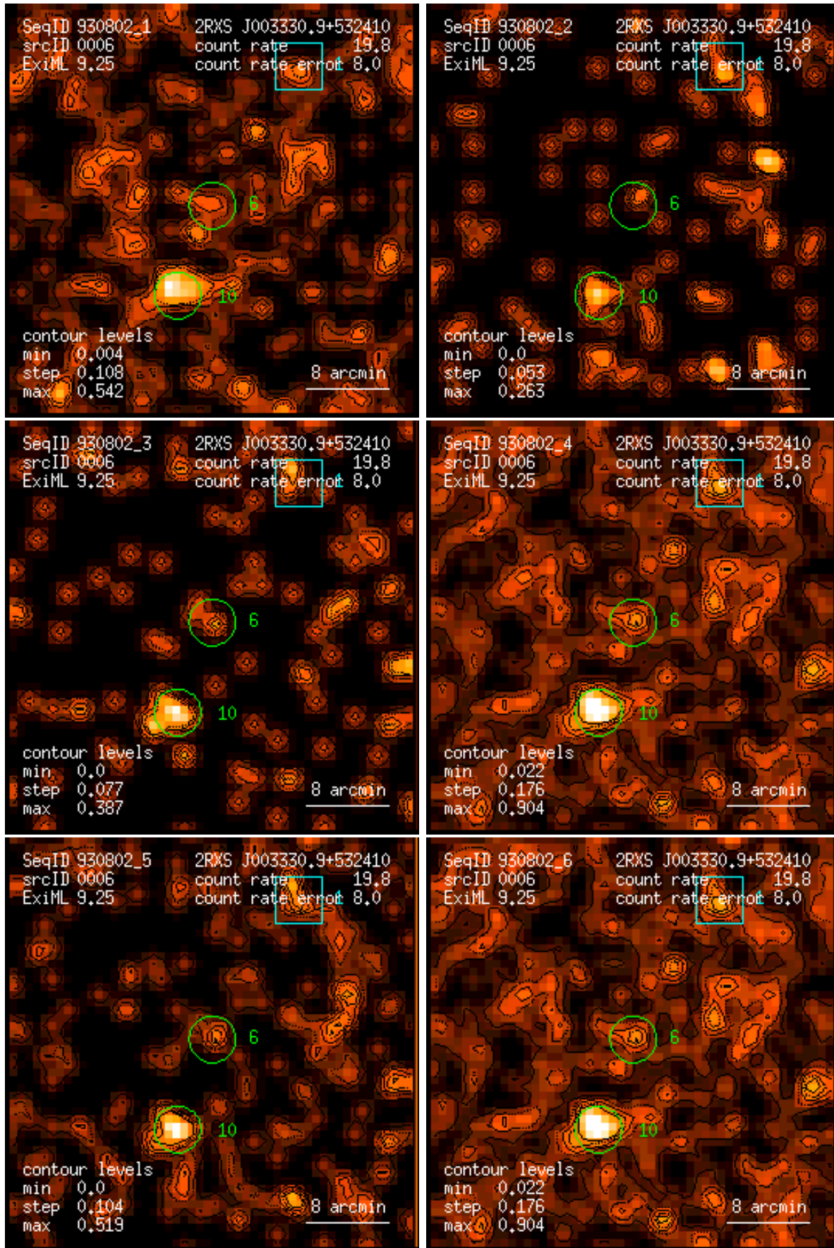
Figure 6: RASS 930802: detection 0006: band rate images, Gaussian filter: (1) PSPC channels 11 – 41, (2) 52 – 90, (3) 91 – 201, (4) 11 – 235, (5) 52 – 201, (6) 11 – 201. Broad band rates in counts/ks. Band rate contour levels in counts/ks/arcmin 2 .
