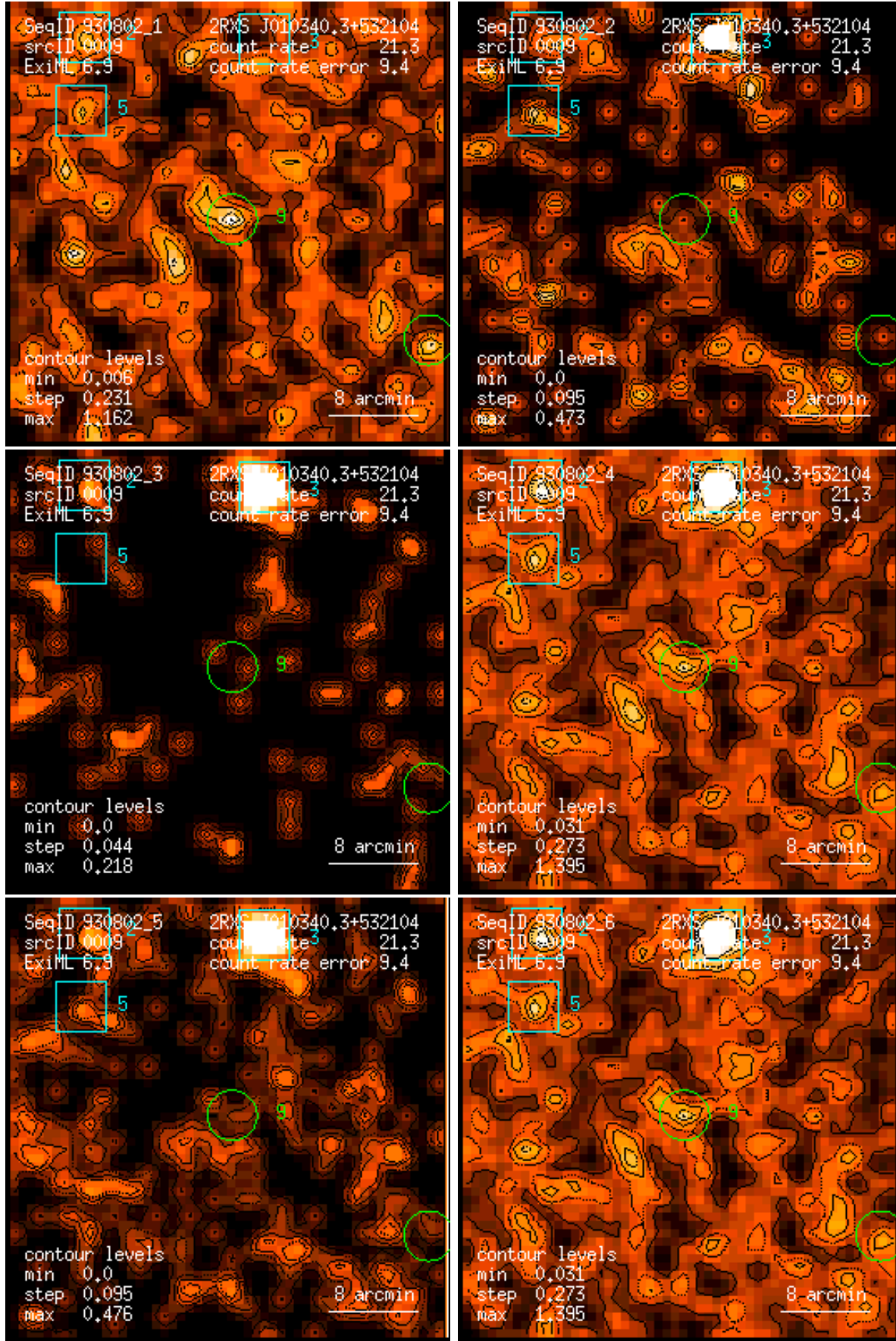
Figure 9: RASS 930802: detection 0009: band rate images, Gaussian filter: (1) PSPC channels 11 – 41, (2) 52 – 90, (3) 91 – 201, (4) 11 – 235, (5) 52 – 201, (6) 11 – 201. Broad band rates in counts/ks. Band rate contour levels in counts/ks/arcmin 2 .
