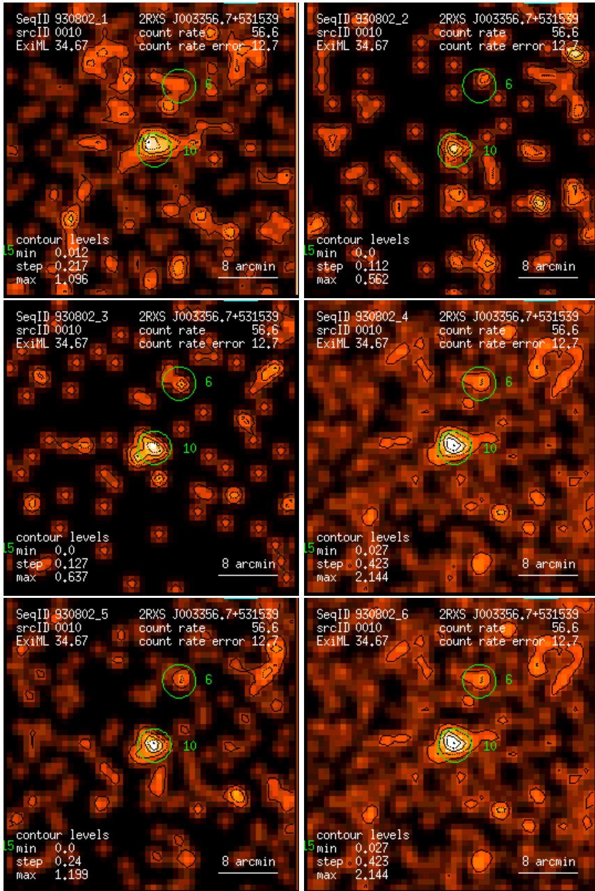
Figure 10: RASS 930802: detection 0010: band rate images, Gaussian filter: (1) PSPC channels 11 – 41, (2) 52 – 90, (3) 91 – 201, (4) 11 – 235, (5) 52 – 201, (6) 11 – 201. Broad band rates in counts/ks. Band rate contour levels in counts/ks/arcmin 2 .
