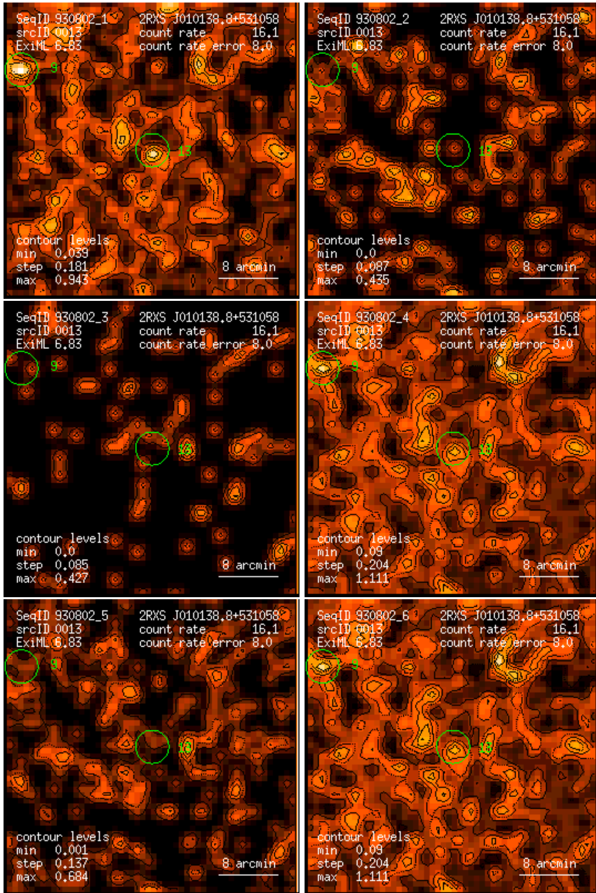
Figure 13: RASS 930802: detection 0013: band rate images, Gaussian filter: (1) PSPC channels 11 – 41, (2) 52 – 90, (3) 91 – 201, (4) 11 – 235, (5) 52 – 201, (6) 11 – 201. Broad band rates in counts/ks. Band rate contour levels in counts/ks/arcmin 2 .
