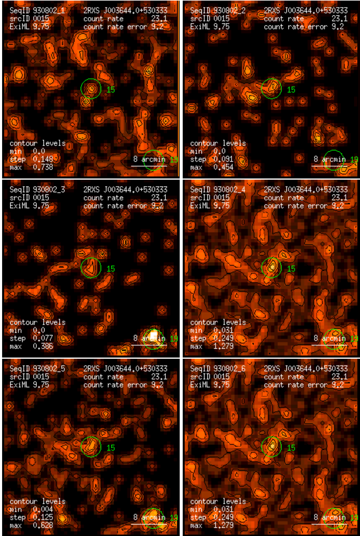
Figure 15: RASS 930802: detection 0015: band rate images, Gaussian filter: (1) PSPC channels 11 – 41, (2) 52 – 90, (3) 91 – 201, (4) 11 – 235, (5) 52 – 201, (6) 11 – 201. Broad band rates in counts/ks. Band rate contour levels in counts/ks/arcmin 2 .
