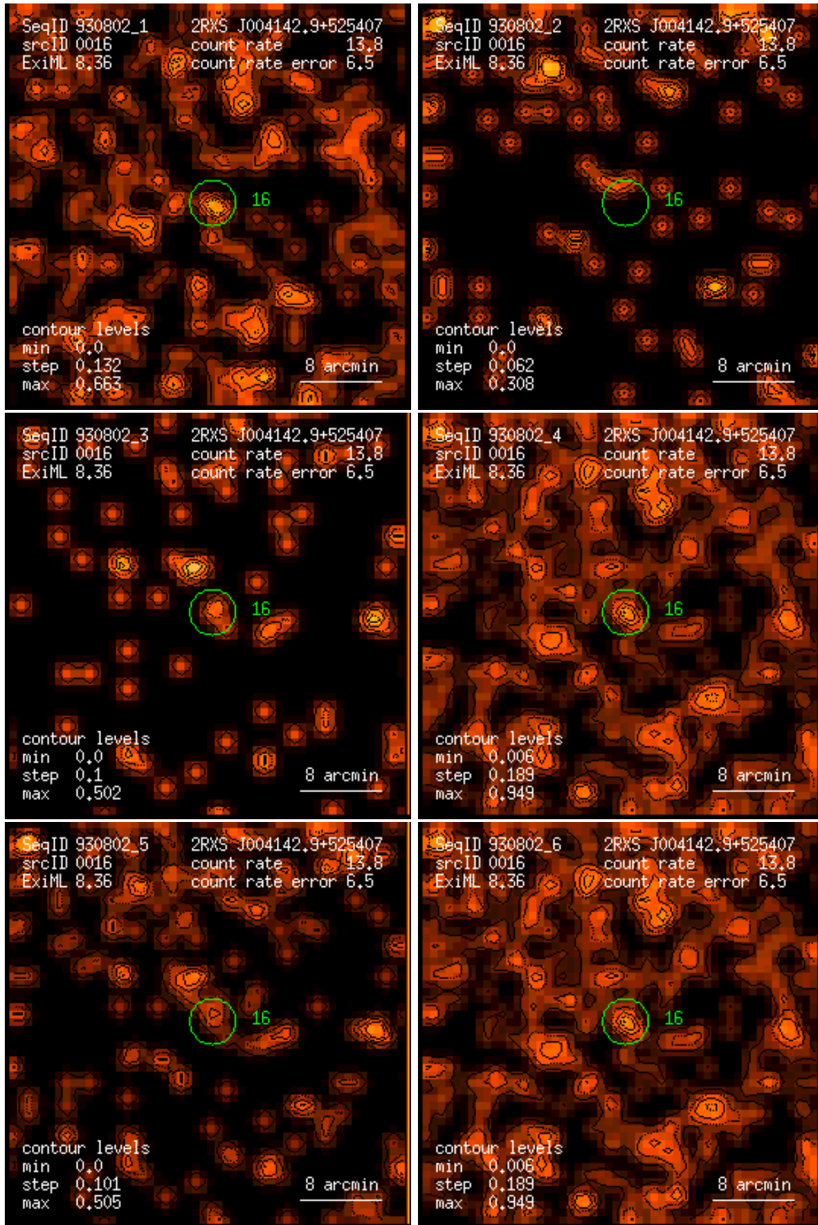
Figure 16: RASS 930802: detection 0016: band rate images, Gaussian filter: (1) PSPC channels 11 – 41, (2) 52 – 90, (3) 91 – 201, (4) 11 – 235, (5) 52 – 201, (6) 11 – 201. Broad band rates in counts/ks. Band rate contour levels in counts/ks/arcmin 2 .
