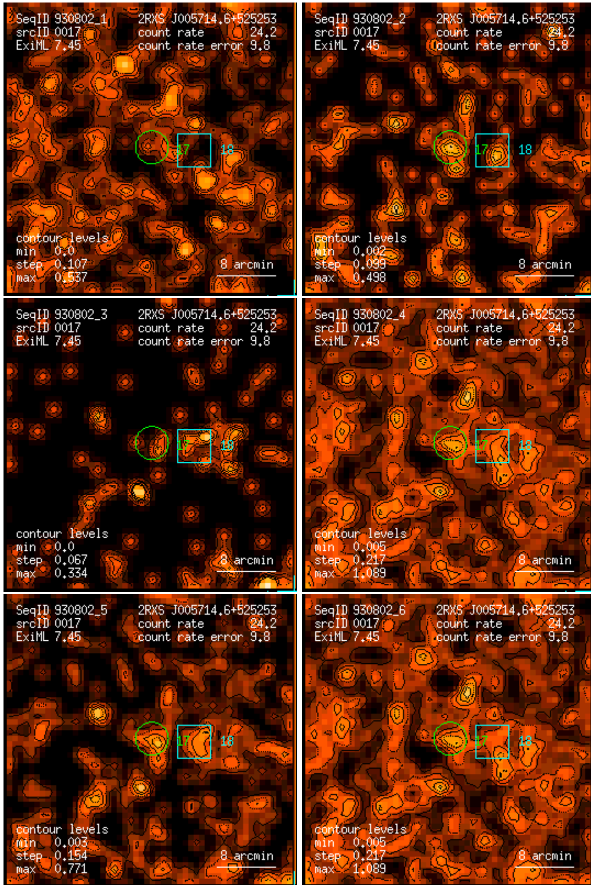
Figure 17: RASS 930802: detection 0017: band rate images, Gaussian filter: (1) PSPC channels 11 – 41, (2) 52 – 90, (3) 91 – 201, (4) 11 – 235, (5) 52 – 201, (6) 11 – 201. Broad band rates in counts/ks. Band rate contour levels in counts/ks/arcmin 2 .
