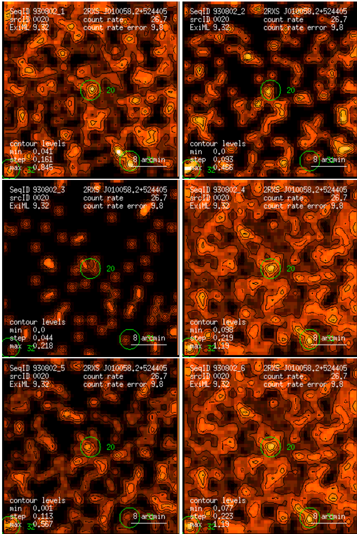
Figure 20: RASS 930802: detection 0020: band rate images, Gaussian filter: (1) PSPC channels 11 – 41, (2) 52 – 90, (3) 91 – 201, (4) 11 – 235, (5) 52 – 201, (6) 11 – 201. Broad band rates in counts/ks. Band rate contour levels in counts/ks/arcmin 2 .
