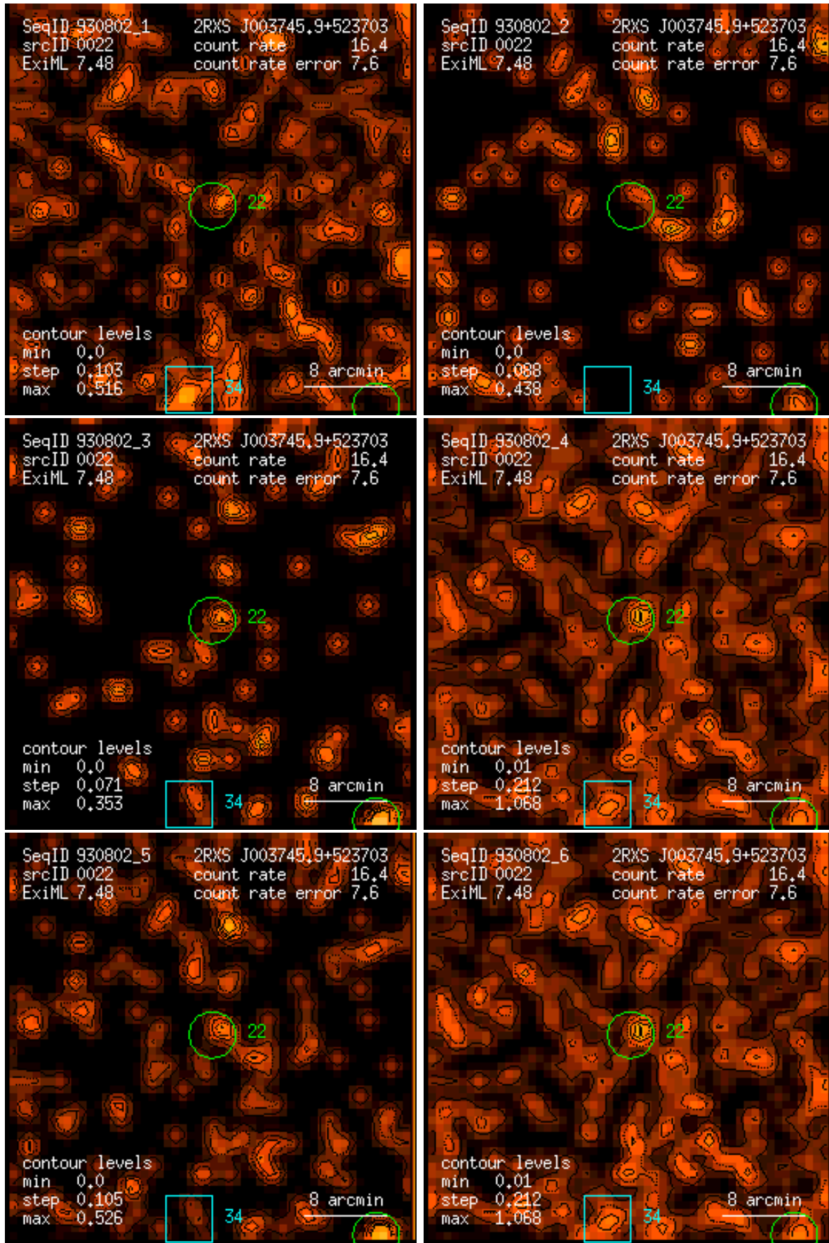
Figure 22: RASS 930802: detection 0022: band rate images, Gaussian filter: (1) PSPC channels 11 – 41, (2) 52 – 90, (3) 91 – 201, (4) 11 – 235, (5) 52 – 201, (6) 11 – 201. Broad band rates in counts/ks. Band rate contour levels in counts/ks/arcmin 2 .
