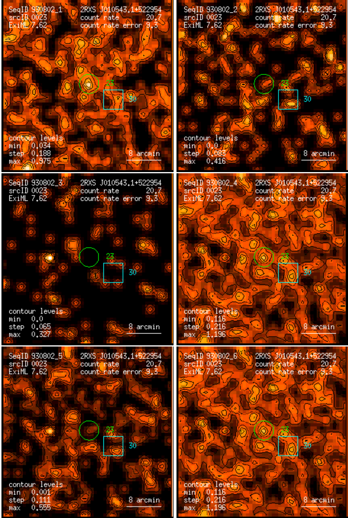
Figure 23: RASS 930802: detection 0023: band rate images, Gaussian filter: (1) PSPC channels 11 – 41, (2) 52 – 90, (3) 91 – 201, (4) 11 – 235, (5) 52 – 201, (6) 11 – 201. Broad band rates in counts/ks. Band rate contour levels in counts/ks/arcmin 2 .
