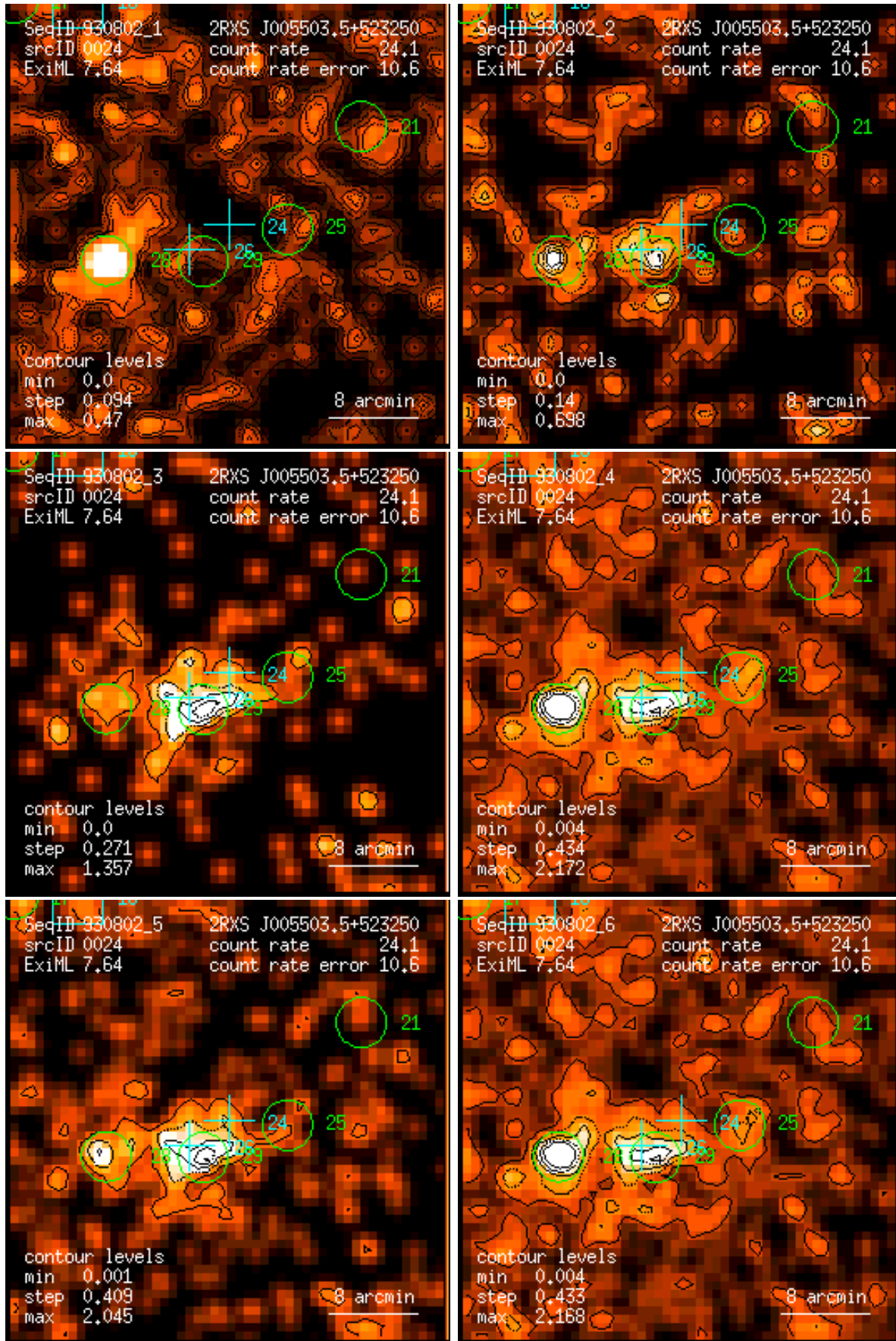
Figure 24: RASS 930802: detection 0024: band rate images, Gaussian filter: (1) PSPC channels 11 – 41, (2) 52 – 90, (3) 91 – 201, (4) 11 – 235, (5) 52 – 201, (6) 11 – 201. Broad band rates in counts/ks. Band rate contour levels in counts/ks/arcmin 2 .
