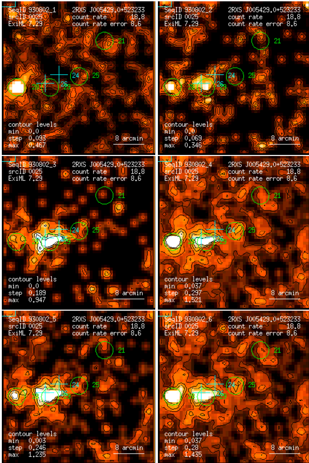
Figure 25: RASS 930802: detection 0025: band rate images, Gaussian filter: (1) PSPC channels 11 – 41, (2) 52 – 90, (3) 91 – 201, (4) 11 – 235, (5) 52 – 201, (6) 11 – 201. Broad band rates in counts/ks. Band rate contour levels in counts/ks/arcmin 2 .
