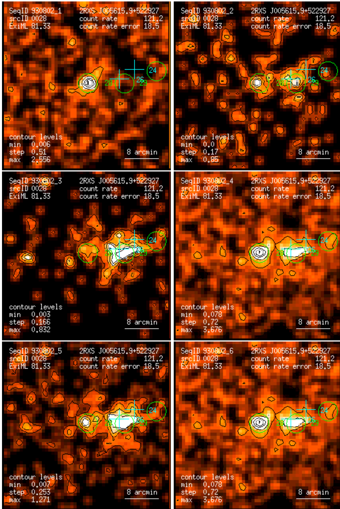
Figure 28: RASS 930802: detection 0028: band rate images, Gaussian filter: (1) PSPC channels 11 – 41, (2) 52 – 90, (3) 91 – 201, (4) 11 – 235, (5) 52 – 201, (6) 11 – 201. Broad band rates in counts/ks. Band rate contour levels in counts/ks/arcmin 2 .
