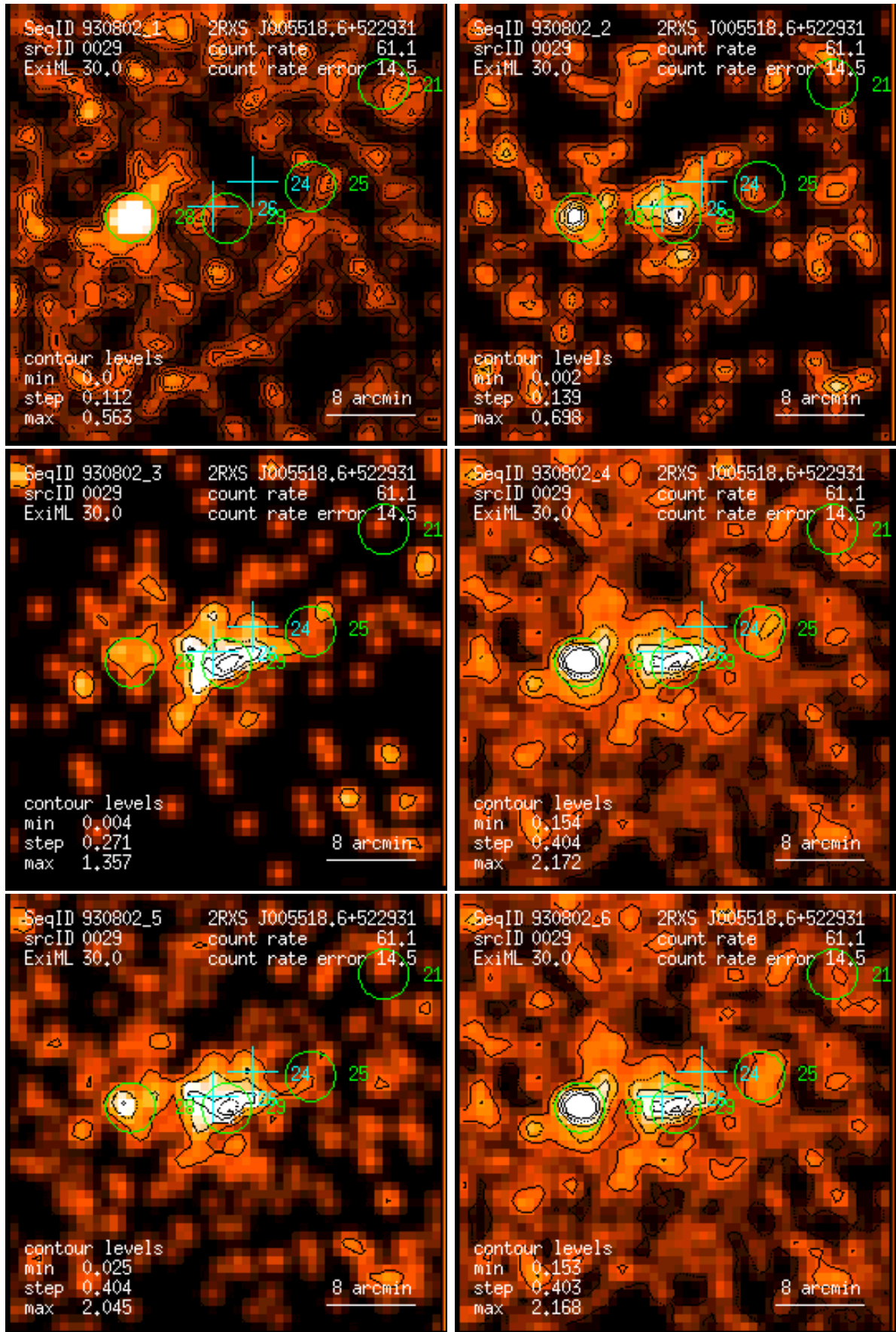
Figure 29: RASS 930802: detection 0029: band rate images, Gaussian filter: (1) PSPC channels 11 – 41, (2) 52 – 90, (3) 91 – 201, (4) 11 – 235, (5) 52 – 201, (6) 11 – 201. Broad band rates in counts/ks. Band rate contour levels in counts/ks/arcmin 2 .
