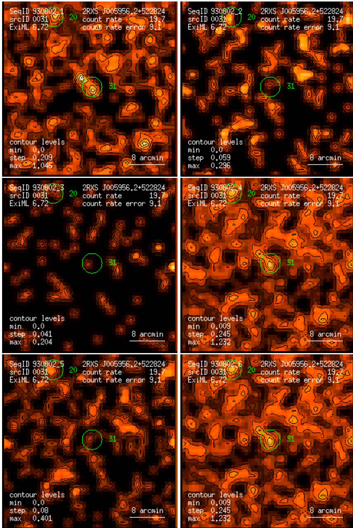
Figure 31: RASS 930802: detection 0031: band rate images, Gaussian filter: (1) PSPC channels 11 – 41, (2) 52 – 90, (3) 91 – 201, (4) 11 – 235, (5) 52 – 201, (6) 11 – 201. Broad band rates in counts/ks. Band rate contour levels in counts/ks/arcmin 2 .
