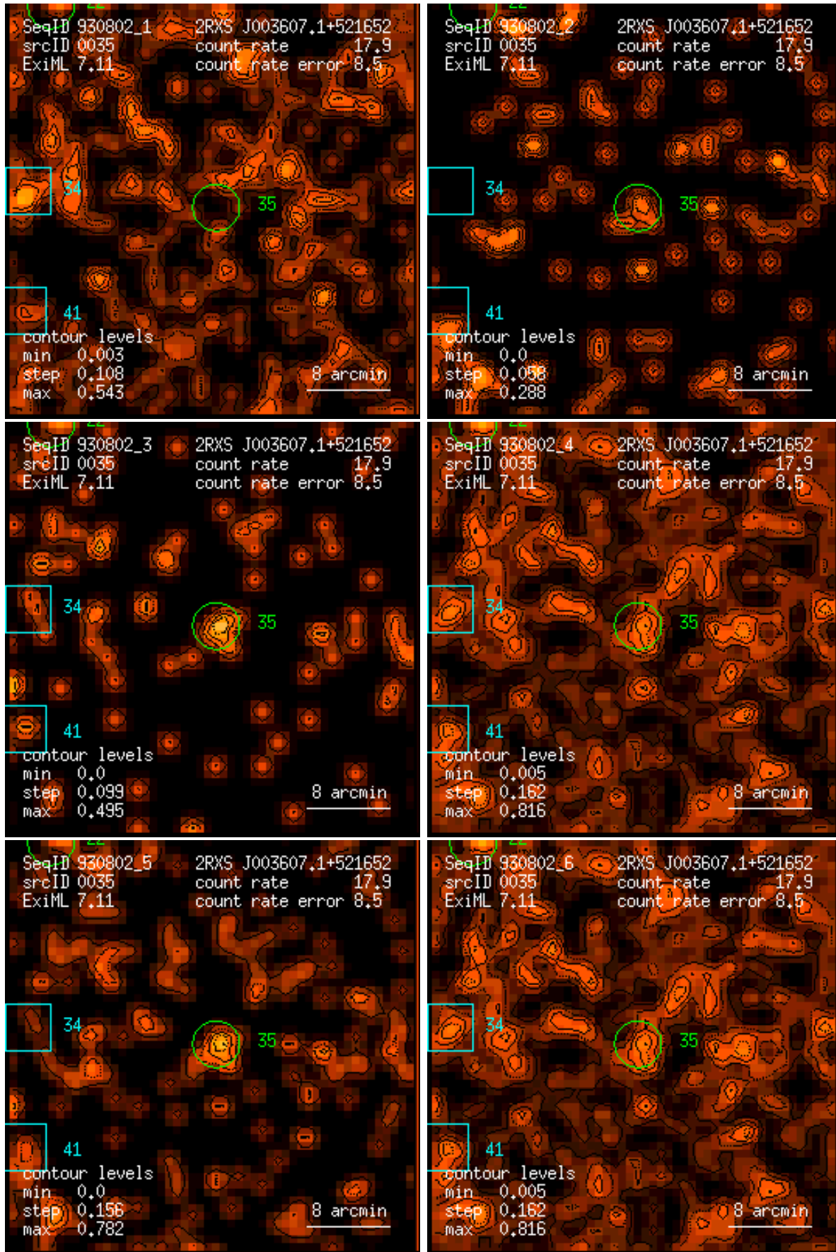
Figure 35: RASS 930802: detection 0035: band rate images, Gaussian filter: (1) PSPC channels 11 – 41, (2) 52 – 90, (3) 91 – 201, (4) 11 – 235, (5) 52 – 201, (6) 11 – 201. Broad band rates in counts/ks. Band rate contour levels in counts/ks/arcmin 2 .
