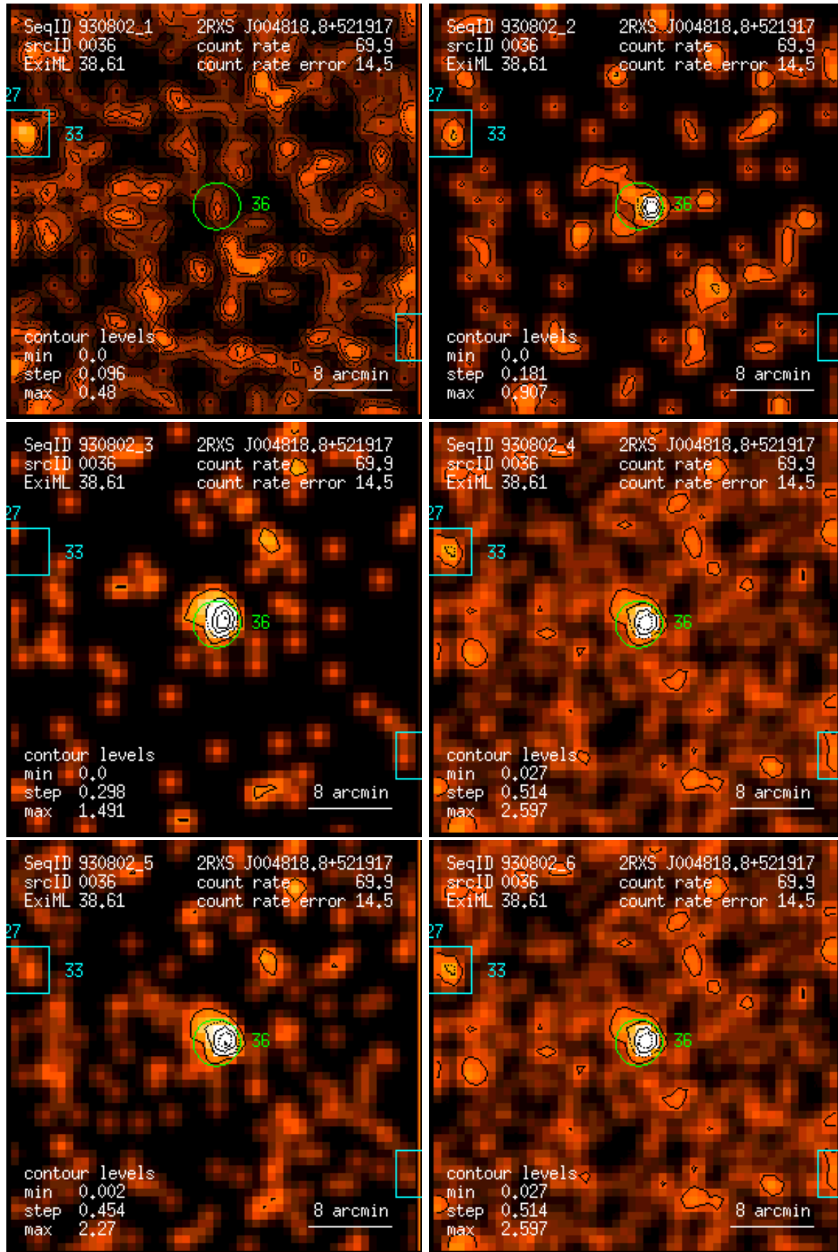
Figure 36: RASS 930802: detection 0036: band rate images, Gaussian filter: (1) PSPC channels 11 – 41, (2) 52 – 90, (3) 91 – 201, (4) 11 – 235, (5) 52 – 201, (6) 11 – 201. Broad band rates in counts/ks. Band rate contour levels in counts/ks/arcmin 2 .
