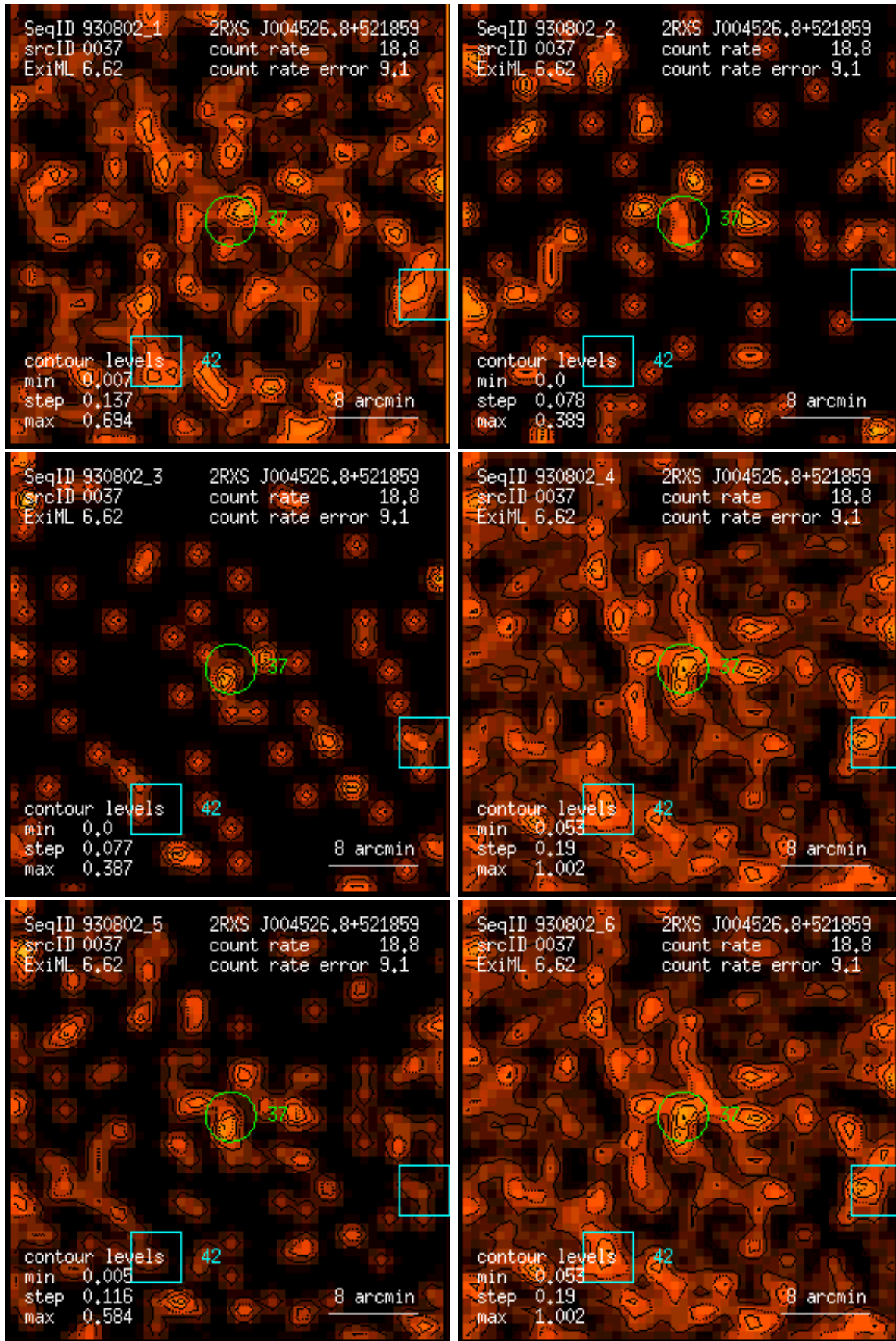
Figure 37: RASS 930802: detection 0037: band rate images, Gaussian filter: (1) PSPC channels 11 – 41, (2) 52 – 90, (3) 91 – 201, (4) 11 – 235, (5) 52 – 201, (6) 11 – 201. Broad band rates in counts/ks. Band rate contour levels in counts/ks/arcmin 2 .
