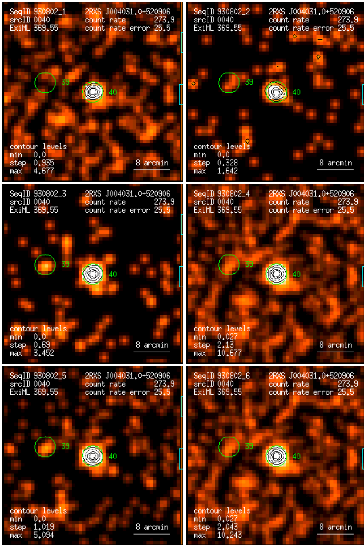
Figure 40: RASS 930802: detection 0040: band rate images, Gaussian filter: (1) PSPC channels 11 – 41, (2) 52 – 90, (3) 91 – 201, (4) 11 – 235, (5) 52 – 201, (6) 11 – 201. Broad band rates in counts/ks. Band rate contour levels in counts/ks/arcmin 2 .
