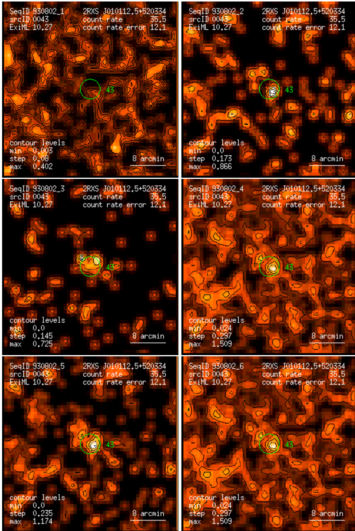
Figure 43: RASS 930802: detection 0043: band rate images, Gaussian filter: (1) PSPC channels 11 – 41, (2) 52 – 90, (3) 91 – 201, (4) 11 – 235, (5) 52 – 201, (6) 11 – 201. Broad band rates in counts/ks. Band rate contour levels in counts/ks/arcmin 2 .
