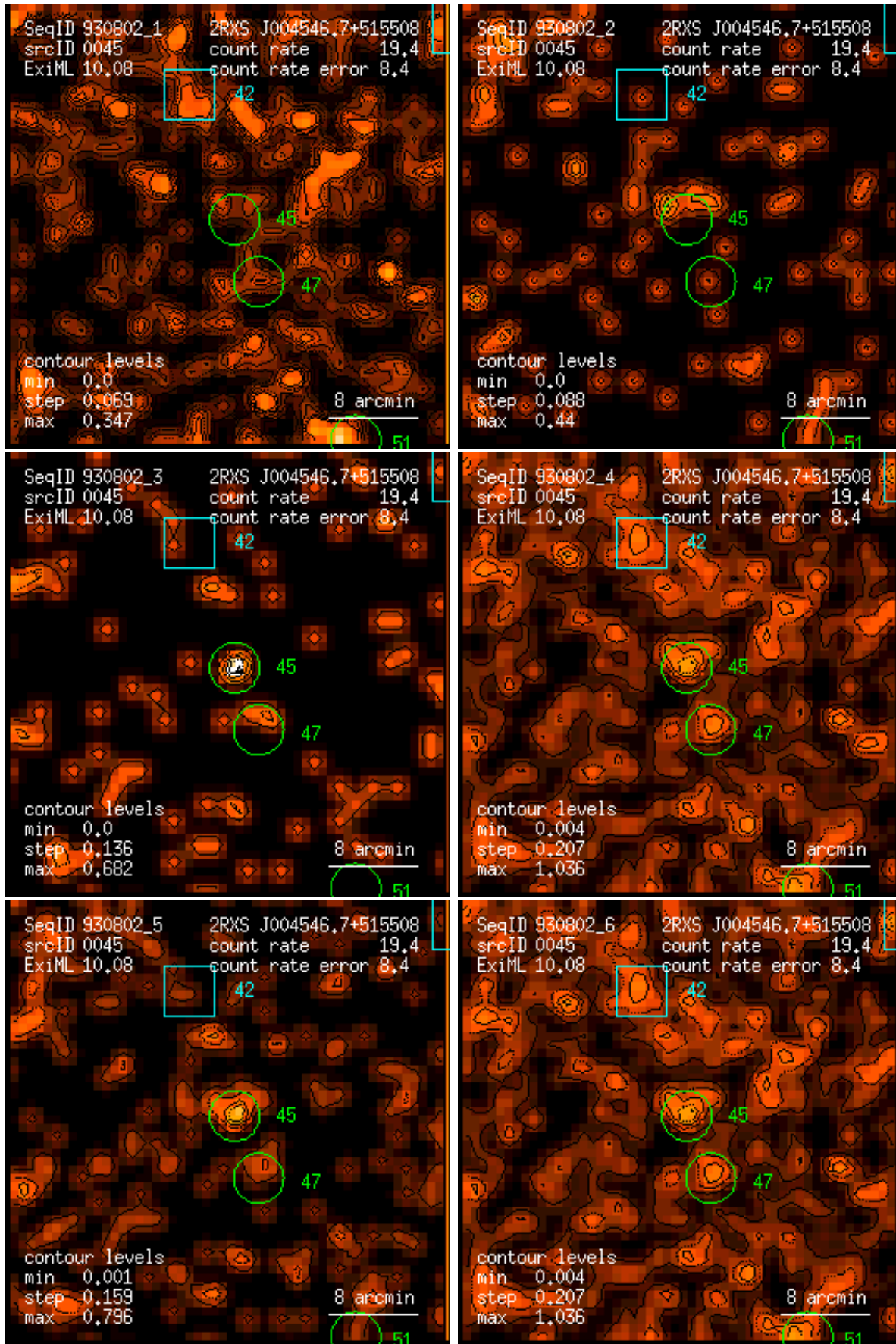
Figure 45: RASS 930802: detection 0045: band rate images, Gaussian filter: (1) PSPC channels 11 – 41, (2) 52 – 90, (3) 91 – 201, (4) 11 – 235, (5) 52 – 201, (6) 11 – 201. Broad band rates in counts/ks. Band rate contour levels in counts/ks/arcmin 2 .
