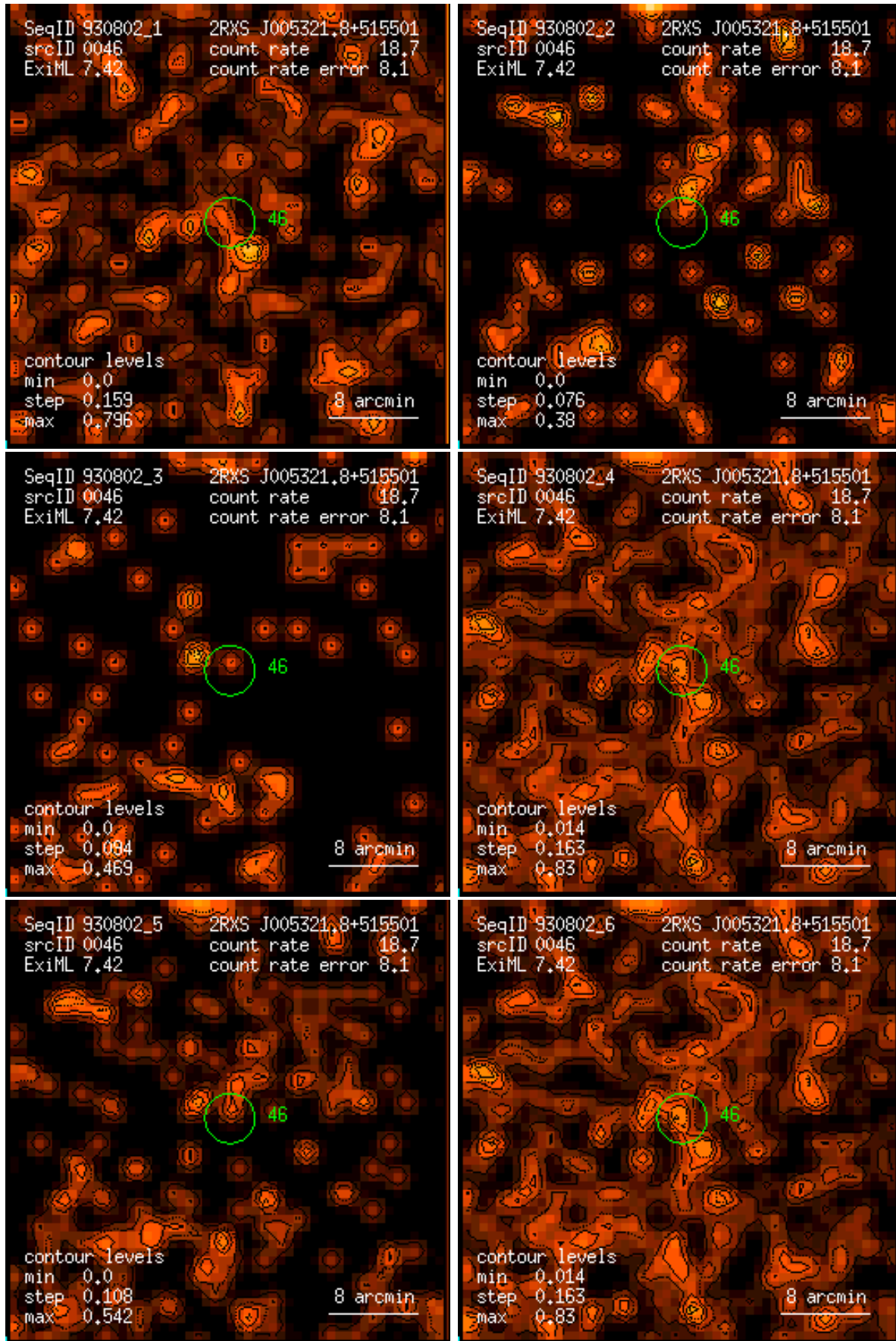
Figure 46: RASS 930802: detection 0046: band rate images, Gaussian filter: (1) PSPC channels 11 – 41, (2) 52 – 90, (3) 91 – 201, (4) 11 – 235, (5) 52 – 201, (6) 11 – 201. Broad band rates in counts/ks. Band rate contour levels in counts/ks/arcmin 2 .
