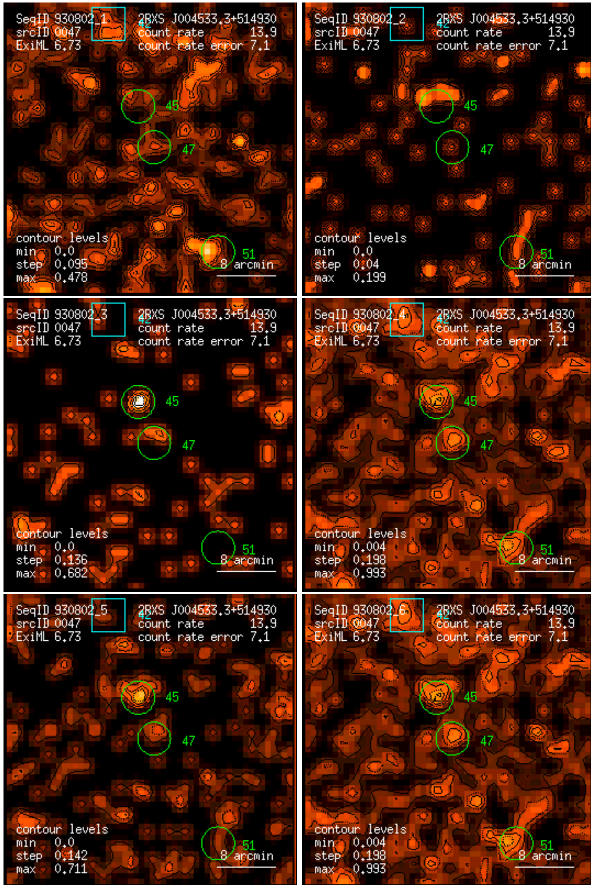
Figure 47: RASS 930802: detection 0047: band rate images, Gaussian filter: (1) PSPC channels 11 – 41, (2) 52 – 90, (3) 91 – 201, (4) 11 – 235, (5) 52 – 201, (6) 11 – 201. Broad band rates in counts/ks. Band rate contour levels in counts/ks/arcmin 2 .
