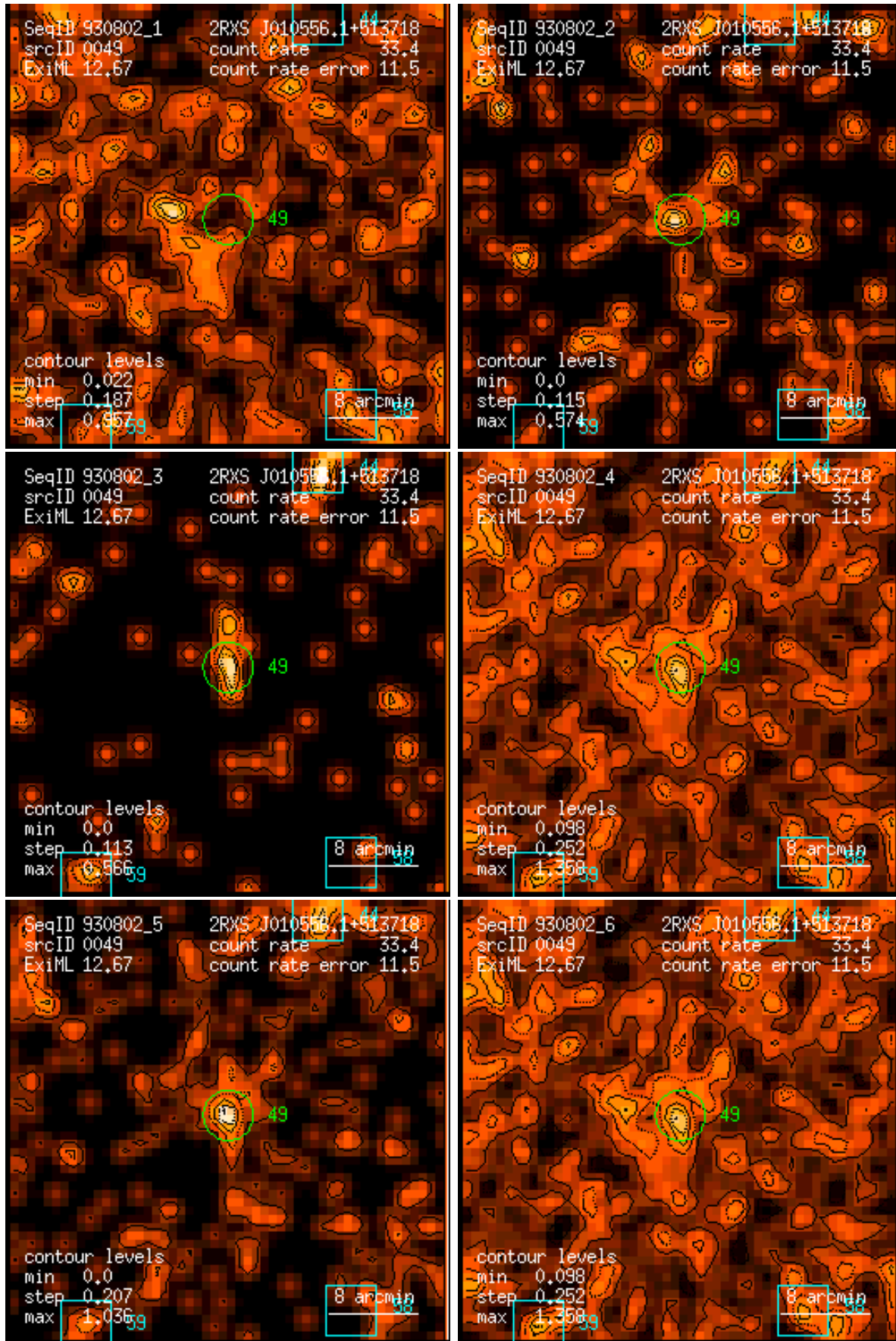
Figure 49: RASS 930802: detection 0049: band rate images, Gaussian filter: (1) PSPC channels 11 – 41, (2) 52 – 90, (3) 91 – 201, (4) 11 – 235, (5) 52 – 201, (6) 11 – 201. Broad band rates in counts/ks. Band rate contour levels in counts/ks/arcmin 2 .
