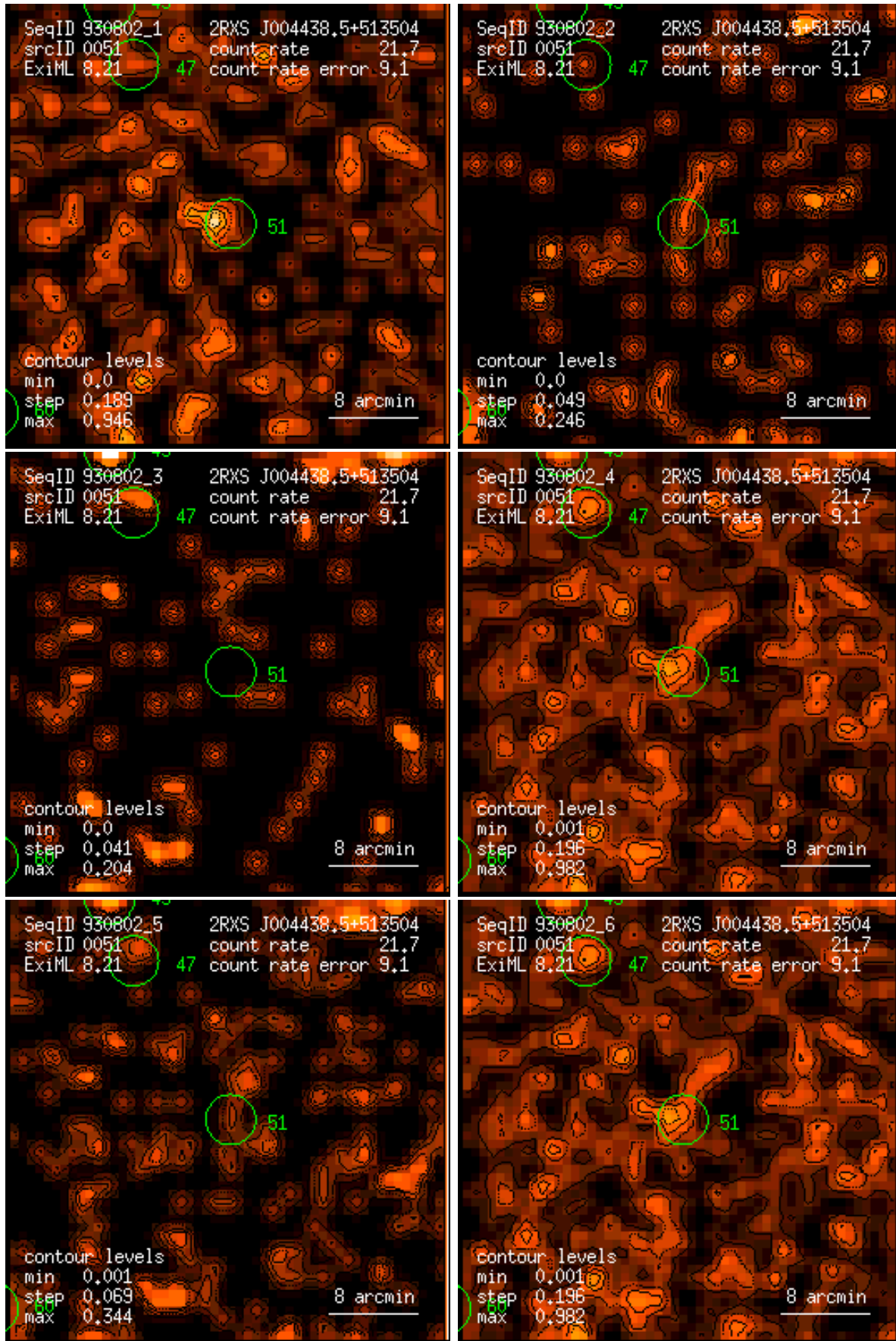
Figure 51: RASS 930802: detection 0051: band rate images, Gaussian filter: (1) PSPC channels 11 – 41, (2) 52 – 90, (3) 91 – 201, (4) 11 – 235, (5) 52 – 201, (6) 11 – 201. Broad band rates in counts/ks. Band rate contour levels in counts/ks/arcmin 2 .
